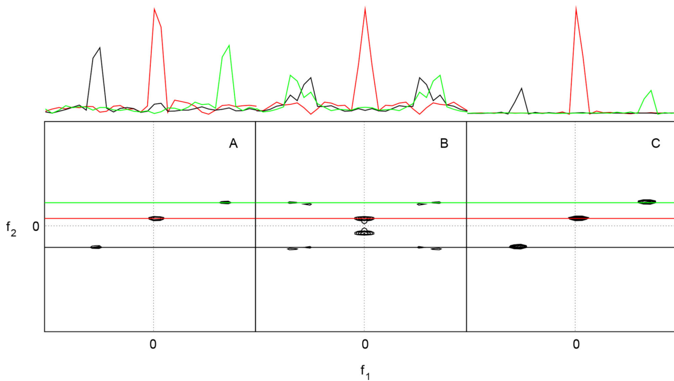
Figure 2. Two-dimensional cross-sections from a four-dimensional N,C-NOESY spectrum, obtained from (A) uniformly sampled hypercomplex (States-Haberhorn-Ruben) data, (B) real values only in the indirect dimensions, and (C) using random phase detection. One-dimensional cross-sections at the frequencies depicted by colored lines crossing the contour plots are depicted at the top. Reprinted with permission from Maciejewski et al. (2011). 46
