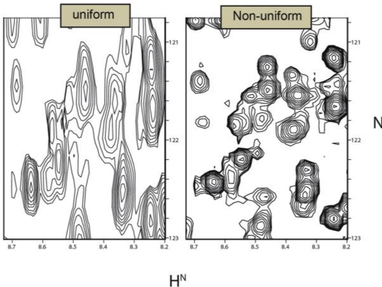
Figure 9. Comparison of a spectrum obtained using uniform sampling and conventional DFT processing (left) with a spectrum obtained using the same number of samples in the indirect dimension (the same experiment time) using NUS and FM processing (right). Adapted from Fig. 1 of Hyberts et al. (2014) 94 . Reprinted with permission.
