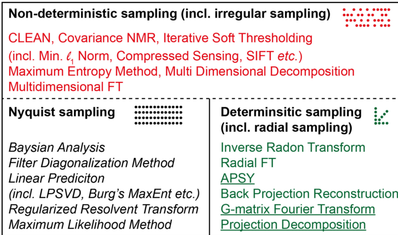
Figure 4. Relationships among different methods used for speeding up NMR data acquisition. Processing methods are categorised based on the type of data they are applicable to. The dotted line indicates that the methods appropriate for non-deterministic sampling are also applicable to the other types of sampling, whereas the converse is not true. Parametric methods are italicised and post-processing methods are underlined.
