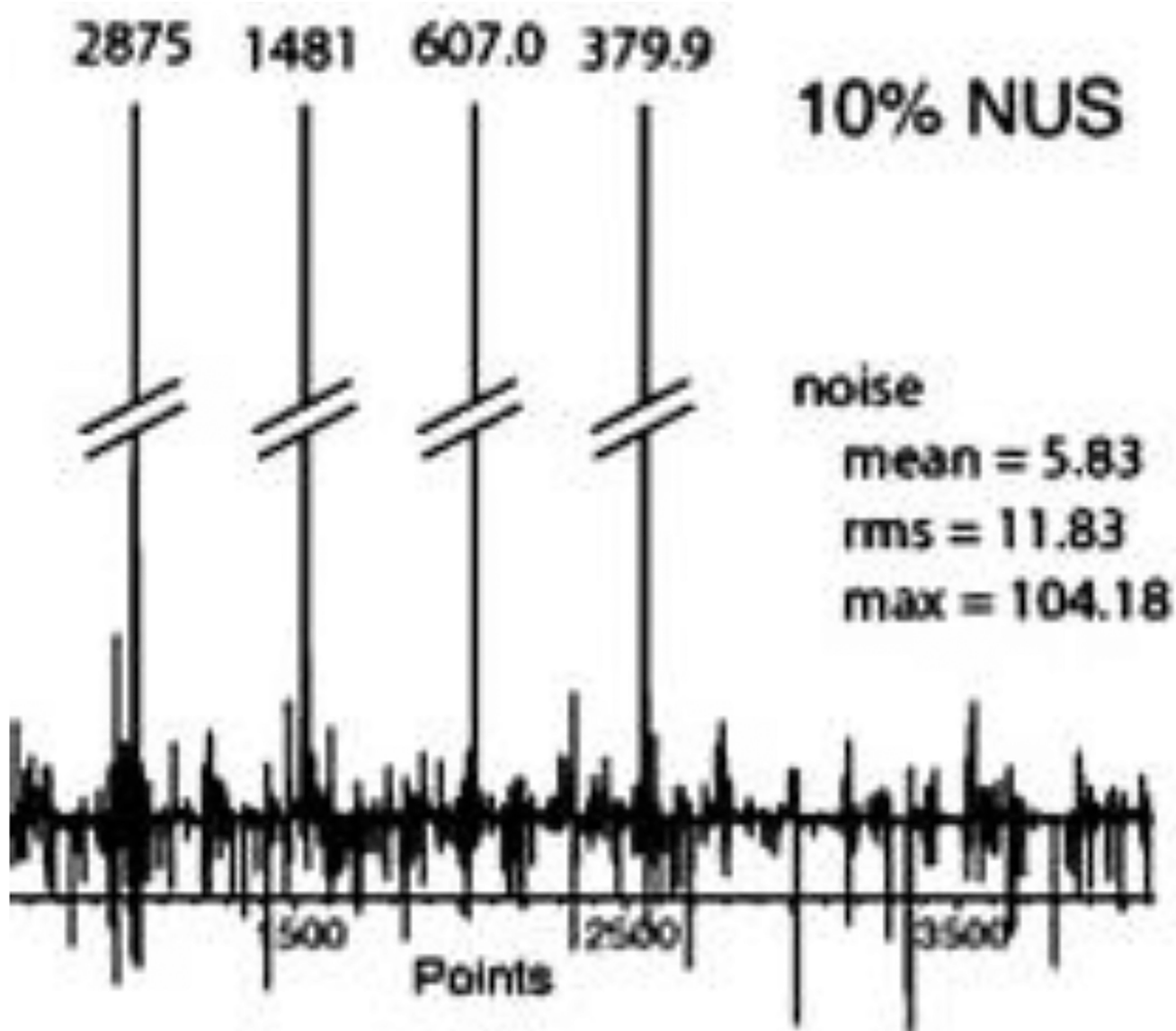
Figure 11. IST spectral reconstruction from NUS data illustrating the non-Gaussian (spiky) noise distribution. Reprinted with permission from Fig. 3D in Stern et al. 96 .
