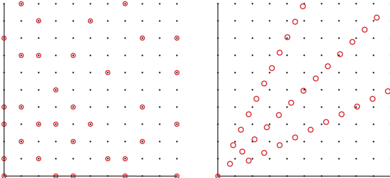
Figure 6. Sampling grid showing on- and off-grid sampling of the same number of points (circles). The off-grid samples are according to radial sampling and the on-grid samples are distributed randomly. The distances between the radial points are sufficient to reconstruct the same spectral window as the underlying grid (black dots) without aliasing.
