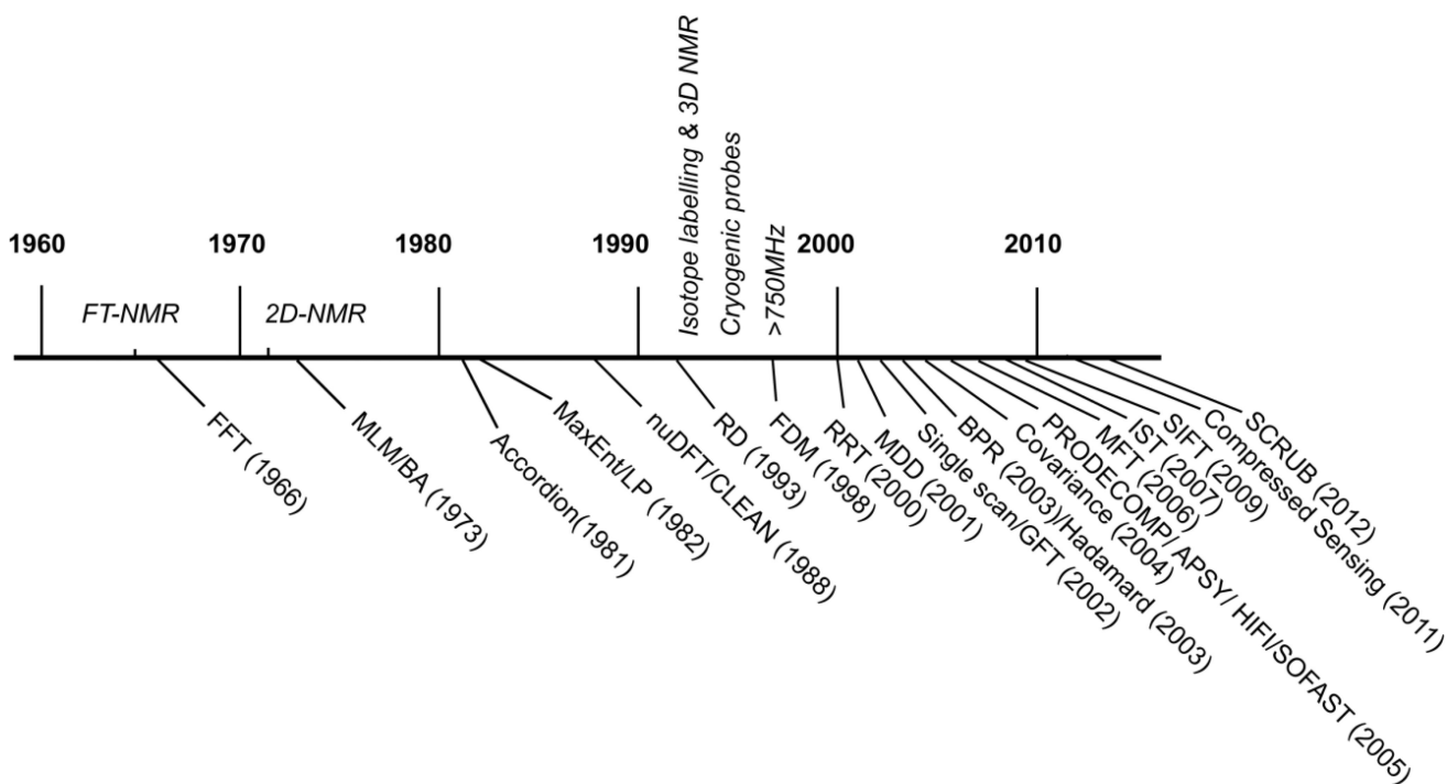
Figure 3. A timeline showing the introduction of various NMR methods aimed at speeding up NMR data acquisition (below the horizontal line). Entries above the timeline refer to fundamental advances in NMR spectroscopy that indirectly impacted or enabled these methods.
