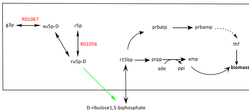
Fig. 5. Knockout targets R01067 and R01056 are shown in red. Identified knockout targets are connected to D-ribulose-1,5-bisphosphate production. The engineered enzymatic reaction is colored in green. Knockouts improve the production of D-ribulose-1,5-bisphosphate from ru5p-D through the engineered enzymatic reaction. (For interpretation of the references to color in this figure legend, the reader is referred to the web version of this article).
