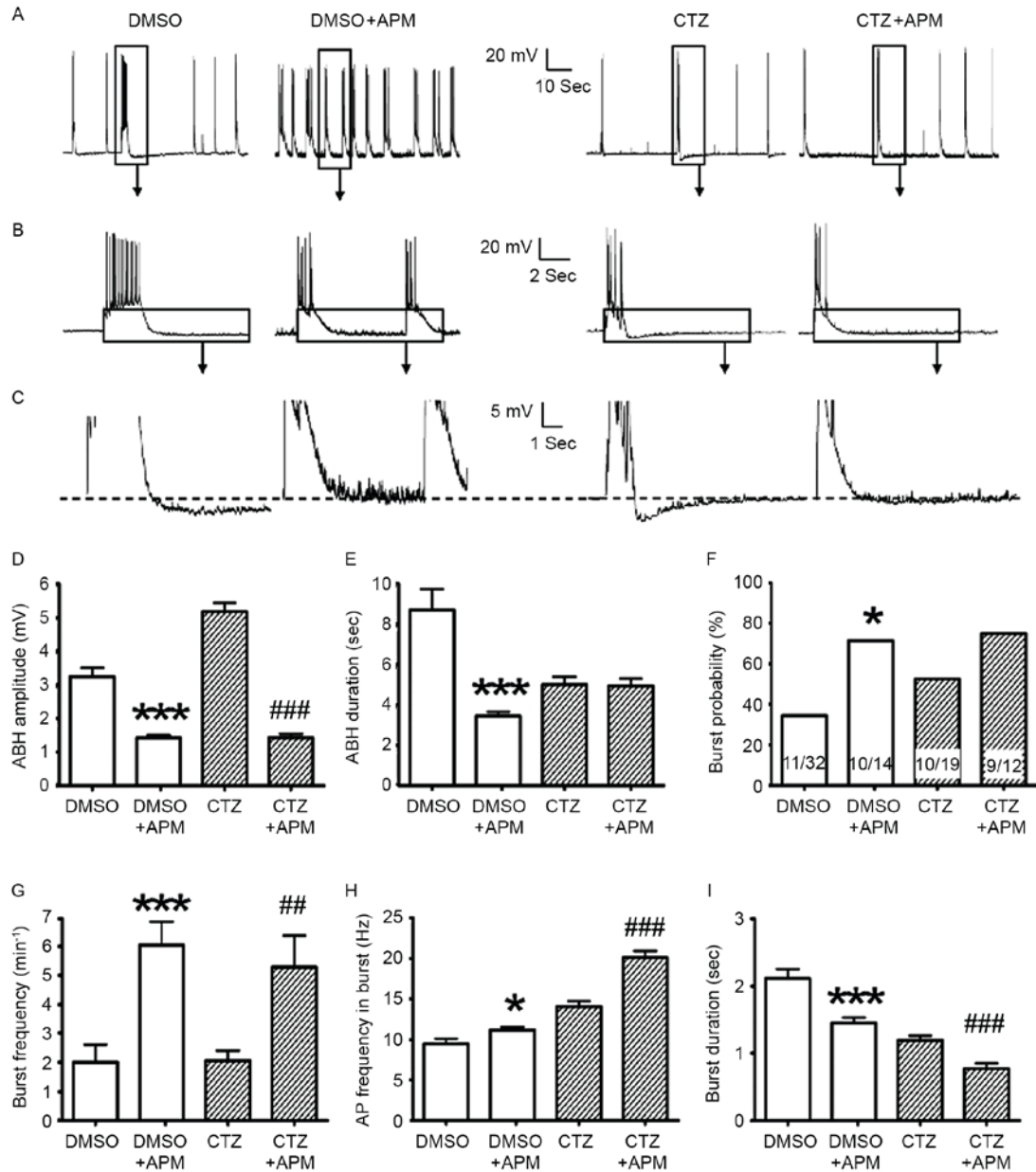
Figure 3. APM impaired ABH; however, it also enhanced burst activities. (A-C) Comparisons between the original recording traces with and without 500 nM APM in the control and 5 \mu M CTZ group for 2 h. The boxes indicate the area that has been enlarged in the subsequent images. (D) APM significantly suppressed the amplitude of ABH in the control group (n=47 without APM; n=64 with APM) and the CTZ group (n=35 without APM; n=61 with APM). (E) APM reduced the duration of ABH in the control group; however, this was not observed in the CTZ group. (F) APM increased the percentage of neurons exhibiting burst activities in the control group; however, not in the CTZ group. The numbers written in the bars represent the number of cells (number with burst activities/total number). (G) APM significantly increased the burst number per minute, in the control group (n=11 without APM; n=10 with APM) and the CTZ group (n=10 without APM; n=9 with APM). (H) AP frequency in burst increased with the application of APM, in the control and CTZ groups. (I) Burst duration significantly decreased in the control and CTZ groups when the bath solution contained APM. Data in D, E, H and I represent the number of burst activities, whereas that in (G) represent the number of neurons. Data are presented as the mean \pm standard error mean. *P<0.05, ***P<0.001 DMSO vs. DMSO + APM; ##P<0.01, ###P<0.001 CTZ vs. CTZ + APM. APM, apamin; ABH, after burst hyperpolarization; CTZ, cyclothiazide; AP, action potential.
