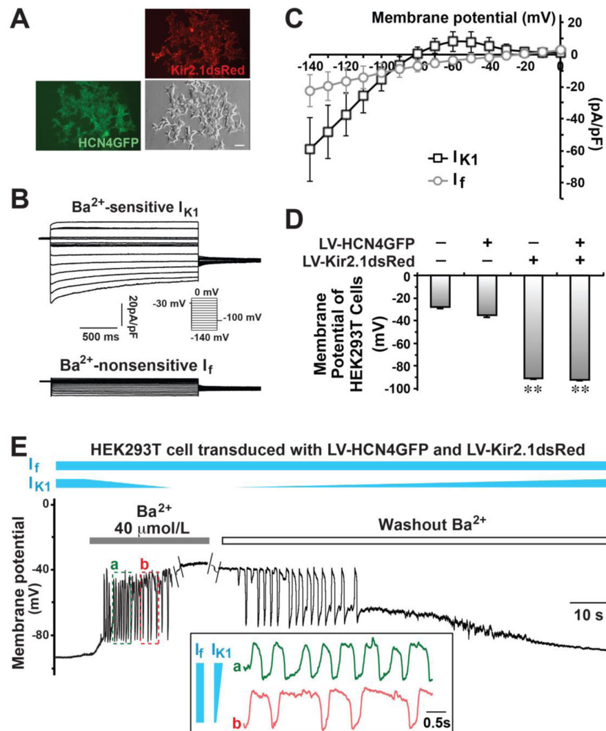
Figure 2. Pacemaker-like rhythmic oscillations of MP could be generated by I_{K1} and I_f in bioengineered HEK293T cells
