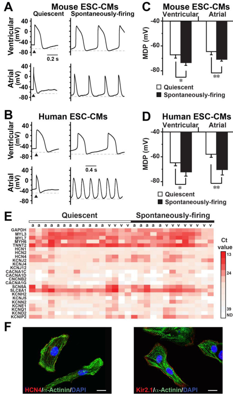
Figure 3. Spontaneously-firing m/hESC-CMs had a more hyperpolarized maximum diastolic potential (MDP)
