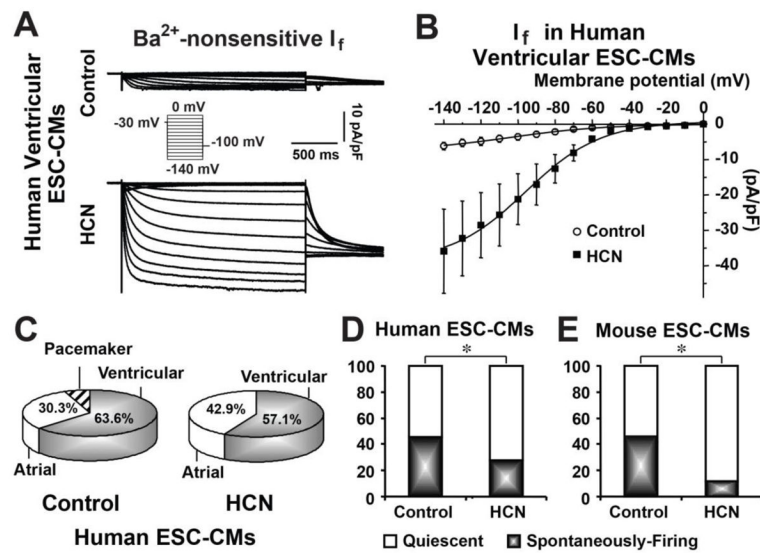
Figure 5. Acute upregulation of I_f suppressed the automaticity of m/hESC-CMs
