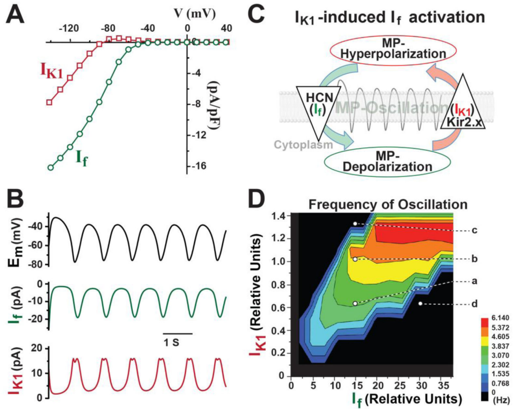
Figure 1. The in silico simulation shows that I_{K1} -induced I_f activation programs rhythmic oscillations of membrane potential (MP)
