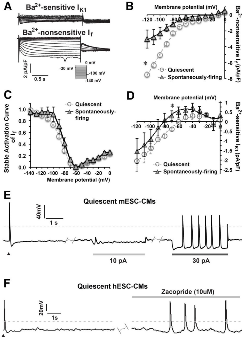
Figure 4. A hyperpolarized MP enhanced the automaticity of quiescent m/hESC-CMs A) Representative I_{K1} and I_f were recorded in ventricular mESC-CMs. B–C) The I–V curve and stable activation curve of I_f in quiescent ( n=5 ) and spontaneously-firing ( n=4 ) ventricular mESC-CMs. D) The I–V curve of I_{K1} showing that spontaneously-firing ventricular mESC-CMs ( n=4 ) displayed a bigger outward current of I_{K1} than quiescent-yet-excitabile ventricular mESC-CMs ( n=5 ). E) Quiescent mESC-CMs ( n=5 ) could spontaneously elicit APs when a proper amount of electrode-injected outward current hyperpolarized the MP. F) The automaticity of quiescent hESC-CMs (6 out of 8, right) was enhanced to fire APs spontaneously after zacopride treatment. Dash lines indicate 0 mV, ▲ indicates an electrical stimulation.
