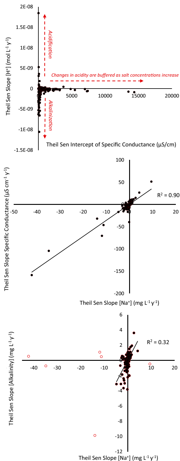
Fig. 6. Rates of change in acidity of stream water (Theil–Sen slopes) are related to initial specific conductance of stream water ( y intercept of slopes) throughout the continental United States. Rates of change in sodium concentrations (Theil–Sen slopes) over time are also strongly related to rates of changes in specific conductance (Theil–Sen slopes) over time. Rates of change in sodium concentrations (Theil–Sen slopes) are related to rates of change in alkalinity concentrations (Theil–Sen slopes) except for 6 out of 232 sites with the most extreme rates of change in sodium concentrations (open circles).
