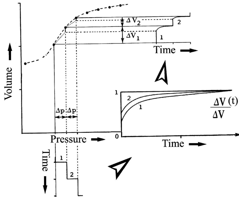
Fig. 9. Schematic representation of how a highly nonlinear pressure-volume curve embodies superposition of consecutive viscoelastic (time dependent) responses to successively imposed pressure steps. V(t) , time-dependent change in volume.
