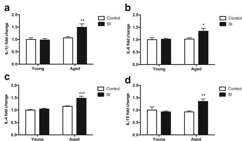
Fig. 4 Brain cytokines levels long term after episodic inflammation. Brain cytokines IL-1 \beta (a), IL-6 (b), IL-4 (c), and IL-10 (d) were measured in young and aged mice naïve (control) and after episodic systemic inflammation (SI). All cytokines measured were significantly elevated in the brains of aged mice after SI. Data were plotted as means \pm SEM ( N = 8 per group, samples collected from 3 independent experiments). Statistical analysis with two-way ANOVA with Bonferroni posttest (* P < 0.05 , ** P < 0.01 , *** P < 0.001 )
