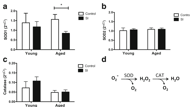
Fig. 6 Brain antioxidant enzymes are downregulated by age and episodic inflammation. Real-time PCR analysis of gene expression was carried out with whole brain mRNA from young and aged mice, naïve (control) or after episodic systemic inflammation (SI). a SOD1 gene expression is significantly decreased in the brain of aged mice after SI. b SOD2 gene expression is not altered by age or SI. c Catalase gene expression is not altered by SI. Data were plotted as means ± SEM (N = 5 to 7 per group). d Chemical reactions of superoxide dismutase (SOD) and catalase (CAT) converting anion superoxide (O 2 - ) into hydrogen peroxide (H 2 O 2 ), oxygen (O 2 ), and water (H 2 O). Statistical analysis with Mann Whitney test (*P < 0.05)
