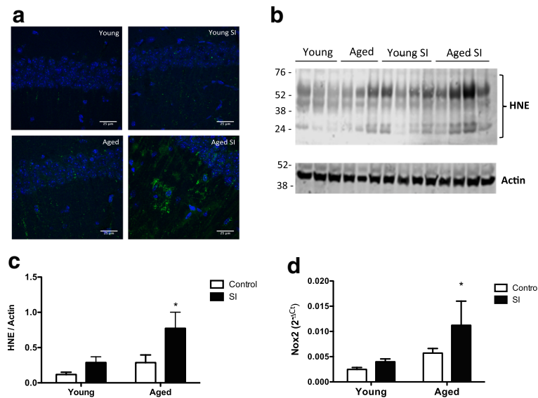
Fig. 5 Oxidative stress is associated with increased Nox2 expression in the aged brains after episodic inflammation. a Confocal images showing increased 4-hydroxynonenal (HNE) immunostaining in the hippocampus of aged mice after SI. Scale bar = 25 μm. b Western blots for HNE protein adducts show increased content of oxidized protein in the brains of aged mice after SI. Molecular weights shown in kilodaltons (kDa). c Quantification of HNE western blot bands intensity, normalized by actin bands. d Real-time PCR analysis of gene expression was carried out with whole brain mRNA from young and aged mice, naïve (control), and long term after episodic systemic inflammation (SI). Data were plotted as means ± SEM (N = 4–5 per group). Statistical analysis with Mann Whitney test (*P < 0.05 relative to young controls)
