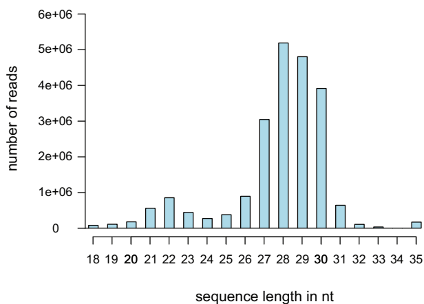
FIG. 2. —Sequence length representation of small RNAs in A. viridis . Distribution of small RNA reads after adapter trimming and quality filtering in one individual sampled from pH 8.2. Two distinct peaks could be observed; first around 22 nt representing both miRNA and siRNA reads, and second around 28 nt representing putative piRNA reads.
