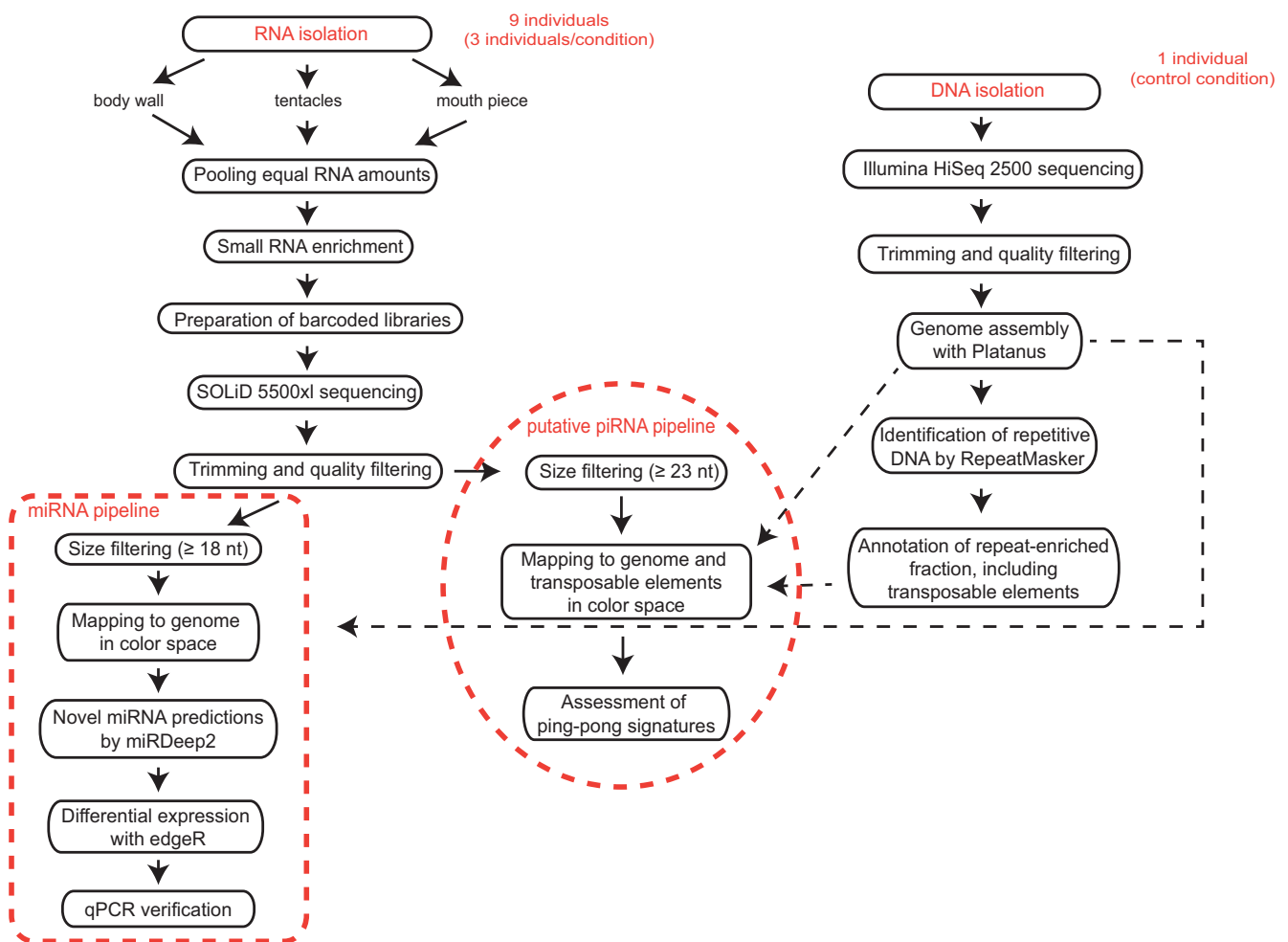
Fig. 1. —Data analysis overview. DNA and RNA were isolated from A. viridis adult polyps sampled from a natural seawater pH gradient (at normal seawater pH 8.2, and at low seawater pH 7.9 and 7.6) off Vulcano Island, Sicily—Italy. Only one polyp (pH 8.2) was used for DNA extraction and was subjected to paired-end sequencing on the Illumina HiSeq2500 platform. Sequencing reads were assembled into a draft genome reference. Subsequently, repeat-enriched regions, including transposable elements were identified and annotated in this assembly. Nine polyps were used for small RNA library preparation and sequencing on the SOLiD 5500xl platform. Sequencing reads were further used for novel miRNA discovery and description of putative piRNA reads.
