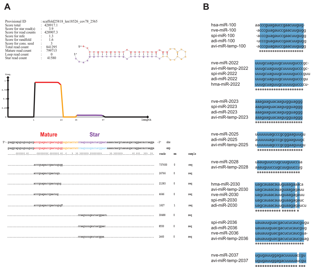
FIG. 3. —Identified miRNAs in A. viridis with similarity to known miRNAs. (A) A typical prediction result from miRDeep2 software tool showing the miRNA precursor, mature and star sequence and their abundances in the sample. Shown is avi-miR-temp-100 precursor with top sequence alignments in the sample for each strand. (B) Alignments of novel miRNAs from A. viridis to known miRNAs from other species. Sequences of our predicted miRNAs from A. viridis (denoted as avi-miR-temp) were aligned to known miRNA sequences from H. sapiens (hsa-miR), N. vectensis (nve-miR), H. magnipapillata (hma-miR), S. pistillata (spi-miR), and A. digitifera (adi-miR). (temp = temporary; miRNAs that are not yet registered in the miRBase).
