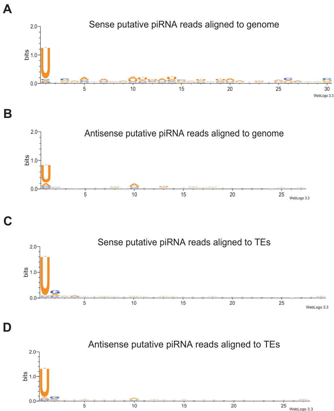
Fig. 6. —Base preferences of putative piRNA reads mapped to various data sets. Shown are base preferences of putative piRNA reads mapping to sense (A, C) and antisense (B, D) strand of genome (A, B) and transposable elements (TEs; C, D). Base preferences did not significantly differ at various pH conditions. Depicted is always one sequence set of specific length from one condition. The Y-axis represents the entropy score for the base bias.
