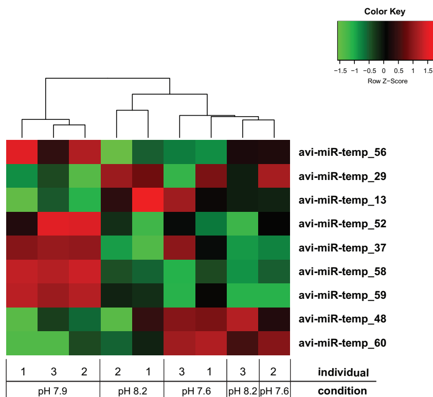
FIG. 5. —Differentially expressed miRNAs under low pH conditions. Nine miRNAs were found differentially expressed among the sampling sites (edgeR, FDR < 0.05). This included two miRNAs detected in all pH conditions studied (avi-miR-temp-13 and 29) and seven miRNAs that could be detected in only one or two different pH conditions. Five miRNAs were differentially expressed between pH 7.6 and 7.9, three downregulated (avi-miR-temp-52, 58, and 59) and two upregulated (avi-miR-temp-48 and 60) at pH 7.6 compared with pH 7.9. Only one miRNA was detected differentially expressed between pH 7.6 and 8.2 (avi-miR-temp-37), and it was upregulated at pH 7.6 compared with pH 8.2. Eight miRNAs were found differentially expressed between pH 7.9 and 8.2, three downregulated (avi-miR-temp-13, 29, and 48) and five upregulated (avi-miR-temp-37, 52, 56, 58, and 59) at pH 7.9 compared with pH 8.2. Differentially expressed miRNAs were hierarchically clustered into heatmap based on counts per million (cpm) and scaled by row.
