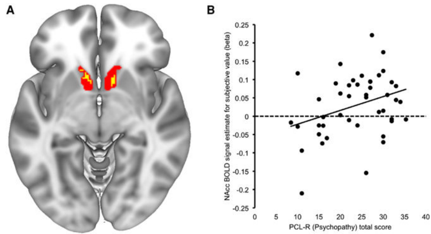
Figure 1. Subjective Value-Related BOLD Activity in the NAcc Tracks Psychopathy Scores (A) The main effect of subjective value across all participants (yellow shading) is overlaid on the nucleus accumbens (NAcc) region of interest (ROI; red shading) used to extract BOLD signal estimates for individual difference analyses (Choi et al., 2012). Small-volume corrected cluster (with bilateral NAcc ROI): p_{\text{FWE(peak-level)}} = 0.043 , peak t value = 3.55, peak MNI coordinate: 12, 12, -6. Whole-brain cluster: peak MNI coordinate: 4, 12, 0; peak t value = 5.94, k = 304 , p_{\text{FWE(peak-level)}} = 0.029 . (B) Scatterplot illustrates the significant positive correlation between psychopathy and subjective value-related BOLD signal within right NAcc.
