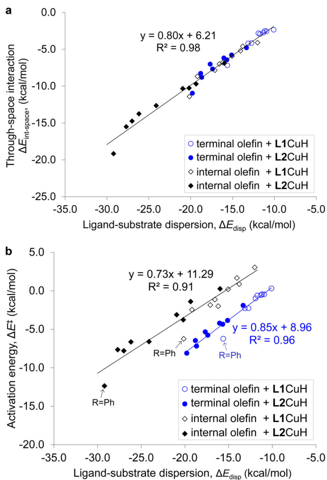
Figure 5. a, Linear correlation between ligand-substrate dispersion ( E_{\text{disp}} ) and total ligand-substrate through-space interaction ( E_{\text{int-space}} ) in the hydrocupration of terminal olefins \text{CH}_2=\text{CHR} and internal olefins \text{trans-CHR}=\text{CHR} ( R = \text{Me, Et, Pr, } i\text{-Pr, } t\text{-Bu, Cy, Bn, CHEt}_2, \text{Ph} ). b, Linear correlations between ligand-substrate dispersion ( E_{\text{disp}} ) and activation energy ( E^\ddagger ).
