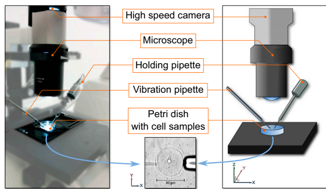
Fig. 1. Illustration of the experiment ( Left : picture; Right : scheme). A cell placed in a Petri dish is held by a holding pipette and vibration is applied using a second pipette attached to a piezo-drive unit. Vibration is applied to the zona pellucida of the oocyte. Images of the cell are acquired by a high-speed camera through a microscope.
