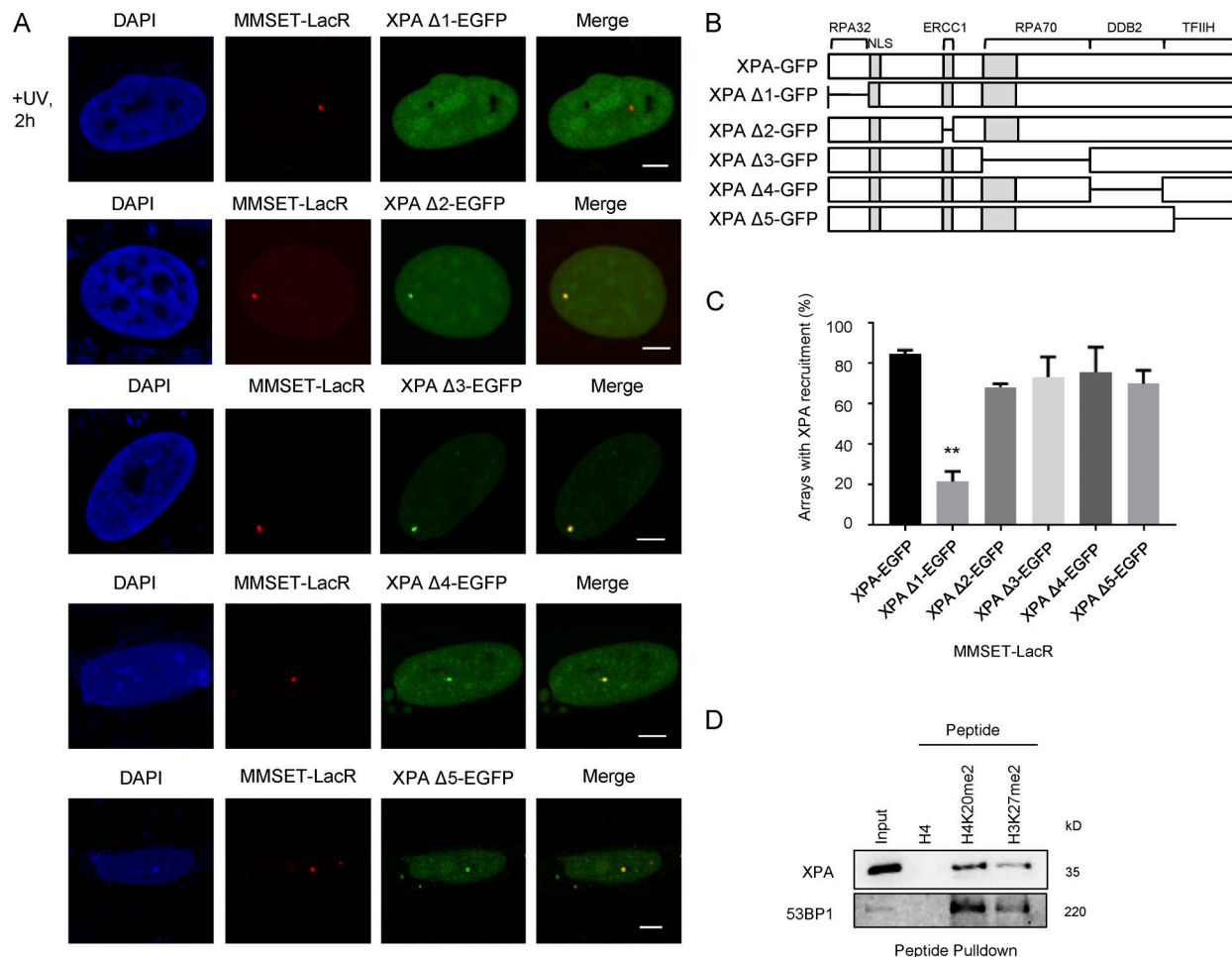
Figure 7. XPA requires the RPA32-binding domain for interaction with H4K20me2. (A) Fluorescence microscopy images showing distribution of XPA deletions ( \Delta 1 – \Delta 5 ) in cells with MMSET-LacR tethered arrays 2 h after UV exposure. (B) Schematic showing the location of the generated XPA deletions. Bars, 5 \mu m. (C) RPA32 binding domain is required for XPA association with H4K20me2. The graph shows a quantification of the number of MMSET-LacR arrays showing recruitment of the indicated GFP tagged XPA deletion, 2 h after UV exposure (mean \pm SEM). Colocalization was measured from three independent experiments, with 30 cells per experiment. Statistical significance was assessed by an unpaired t test. **, P \leq 0.001 . (D) H4K20me2 associates with XPA and 53BP1. Peptide pull-downs with biotinylated H4, H3K27me2, and H4K20me2 peptides and nuclear extracts expressing GFP-XPA. Specific interactions were analyzed by immunoblotting using the indicated antibodies.
