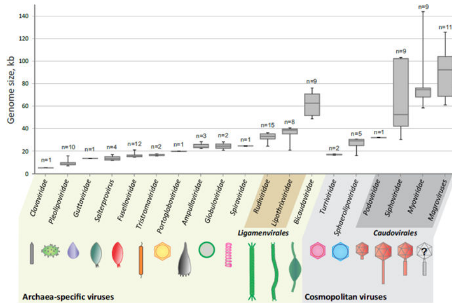
Figure 1. Genome size distribution and morphotypes of archaeal viruses. In the box plot, each box represents the middle 50th percentile of the data set and is derived using the lower and upper quartile values. The median value is displayed by a horizontal line inside the box. Whiskers represent the maximum and minimum values. The number of genomes used for construction of the box plot is indicated for each group of archaeal viruses. The information on the genome sizes was collected from the GenBank records as well as from the published literature (for genomes assembled from metagenomic data). Archaea-specific and cosmopolitan fractions of the archaeal virosphere are indicated with different background colors.
