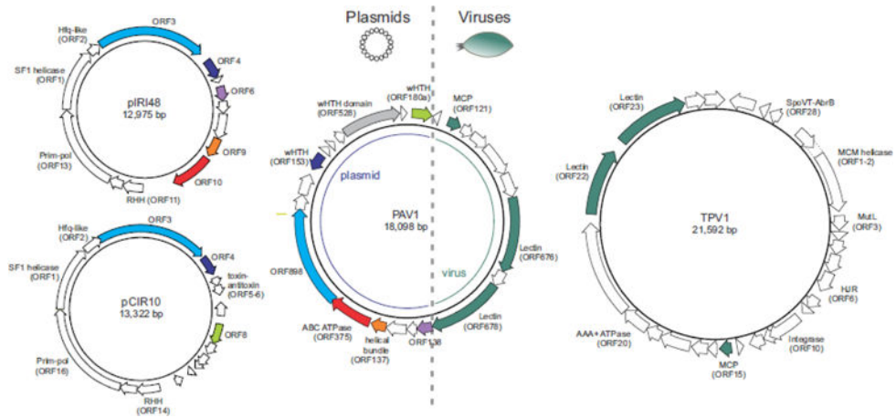
Figure 5. Relationship between thermococcal plasmids and viruses. Homologous genes are colored similarly. PAV1 ORF528, which has homologues in haloarchaeal plasmids, is shaded grey. Note that viruses PAV1 and TPV1 share only genes encoding structural proteins (dark green arrows). Abbreviations, MCP, major capsid protein; SF1, superfamily 1; wHTH, winged helix-turn-helix; RHH, ribbon-helix-helix; HJR, Holliday junction resolvase; prim-pol, primase-polymerase.
