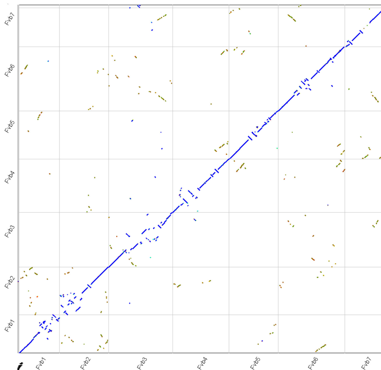
Figure 2: Macrosyntentic comparison of the V2 and V4 F. vesca assemblies. Syntentic gene pairs between V4 (x-axis) and V2 (y-axis) of F. vesca were identified by DAGChainer [44], sorted by chromosome (Fvb1-7), and colored based on their synonymous substitution rate, as calculated by CodeML [45] using SynMap within CoGe [46]. Syntentic “orthologous” regions are colored in blue, and duplicated genes retained from a whole-genome triplication event (At-gamma [47]) in other colors. Regions that were misassembled and incorrectly scaffolded in F. vesca V2 are identified by negatively sloped and repositioned lines.
