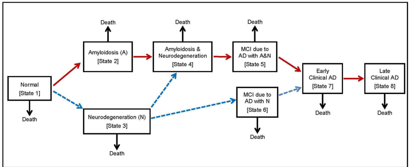
Figure 1. Multistate model of the progression of Alzheimer’s disease through preclinical and clinical disease states.
