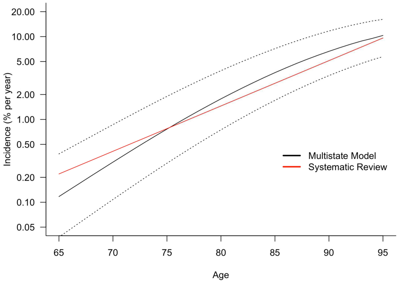
Figure 4. Comparison of age-specific Alzheimer's disease incidence rates expressed as percent per year from a worldwide systematic review [12] (red curve) and from the multistate model (black curve) on a log scale. Also shown are the AD incidence rates from the multistate model based on the series of high and low transition rates that were used in the sensitivity analysis (black dotted curves).
