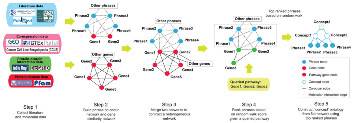
Figure 1. Diagram of our method
