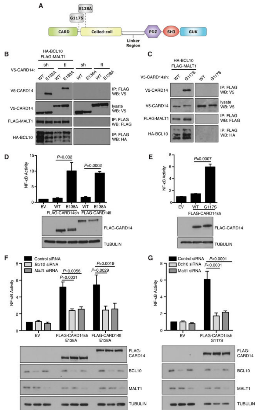
Figure 1. Psoriasis-associated CARD14 mutants require BCL10 and MALT1 to activate NF- \kappa B (A) Schematic of CARD14 domains and psoriasis-associated mutations. (B, C) HEK293 cells were co-transfected with vectors encoding the indicated V5-CARD14 variants (0.1–1.2 \mu g), FLAG-MALT1 (1 \mu g) and HA-BCL10 (0.6–1.2 \mu g). Anti-FLAG immunoprecipitates were immunoblotted with the indicated antibodies. Representative of at least two independent experiments. (D, E) HaCaT keratinocytes were co-transfected with vectors encoding the indicated FLAG-CARD14 variants (0.125–0.2 \mu g) or EV, pNF- \kappa B-Luc and pRL-TK. After 24 h, NF- \kappa B activity was determined by luciferase assay (mean \pm S.E.M. of
