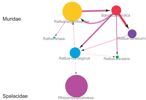
Figure 3. Transmission network of kobuviruses in 7 rodent species. Size of nodes describes the number of kobuviruses from each species. Arrows show the direction of transmission between species; the arrow width indicates per capita transmission rate (exchanges year -1 ). Transmission rates and BF support are given in Supplementary Table S3.
