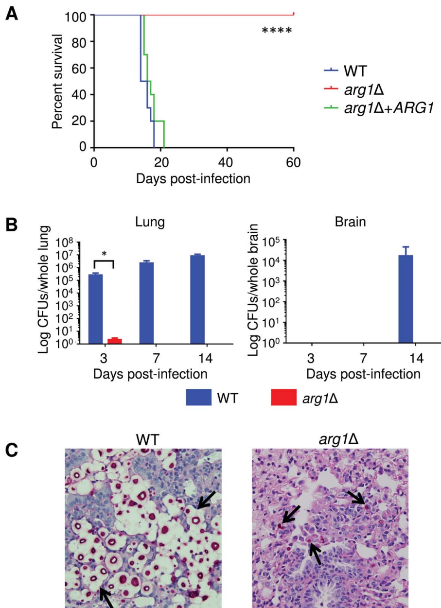
Figure 10. Arg1 is essential for lung colonization and dissemination in a murine inhalation model of cryptococcosis. (A) arg1Δ is avirulent compared to WT and arg1Δ + ARG1. Mice ( n = 10 per strain) were inoculated intranasally with 5 \times 10^5 cells/20 \mu\text{L} and monitored daily. Difference in survival between WT/ arg1Δ + ARG1-infected mice and arg1Δ -infected mice is statistically significant (**** P < 0.0001 ). (B) and (C) arg1Δ infection is rapidly cleared from mouse lung between 3 and 7 days post-infection. Mice ( n = 3 per strain) were inoculated intranasally with 5 \times 10^5 cells/20 \mu\text{L} and sacrificed on the days indicated. Lung and brain were harvested for quantitative culture (CFUs) (B) or histopathological analysis for lung only by Periodic acid–Schiff (PAS) staining (C). In (B), the difference in lung CFUs for WT and arg1Δ -infected mice at day 3 is statistically significant (* P < 0.05 ). In (C), lung histopathology is shown at 3 days post-infection (PAS stain, 40x magnification). In WT-infected lung tissue, arrows indicate cryptococcomas where capsular material is represented by white halos surrounding the cell bodies (stained magenta). In arg1Δ -infected tissue, arrows indicate single acapsular cryptococcal cells.
