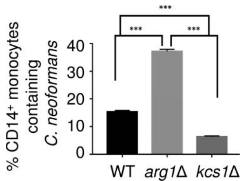
Figure 11. arg1 Δ is more readily phagocytosed by human PBMCs. Results are expressed as the mean % of CD14 + monocytes containing FITC-labelled C. neoformans ± SD (n = 3). Statistical significance is indicated as follows: ***P < 0.001.
