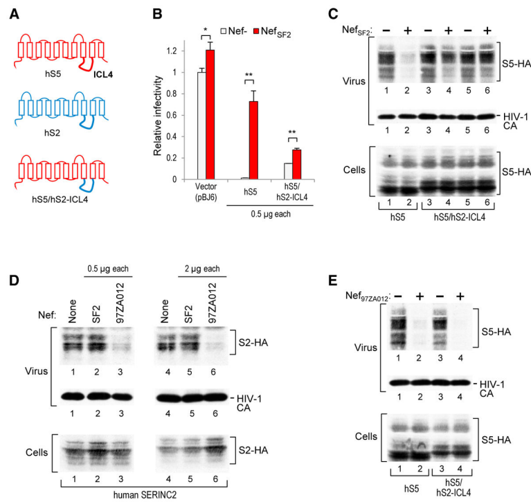
Figure 4. ICL4 of Human SERINC2 Confers Resistance to Nef SF2 , but Not Nef 97ZA012 (A) Schematic illustration of the parental human SERINC proteins and of the chimera examined. (B) Inhibitory activity of human SERINC5 bearing the ICL4 of human SERINC2 on Nef - HIV-1 progeny virion infectivity is largely resistant to Nef SF2 . Bar graphs represent the mean + SD from 3 biological replicates. (C) Western blots showing that the incorporation of the SERINC chimera into Nef - HIV-1 virions is largely unaffected by Nef SF2 expressed in trans . The incorporation of the chimera was analyzed in duplicate to document reproducibility. (D) Western blots showing that the incorporation of human SERINC2 into Nef - HIV-1 virions is unaffected by Nef SF2 but inhibited by Nef 97ZA012 . (E) Western blots showing that Nef 97ZA012 inhibits the incorporation of human SERINC5 bearing the ICL4 of human SERINC2 into Nef - HIV-1 virions. See also Figures S3 and S4.
