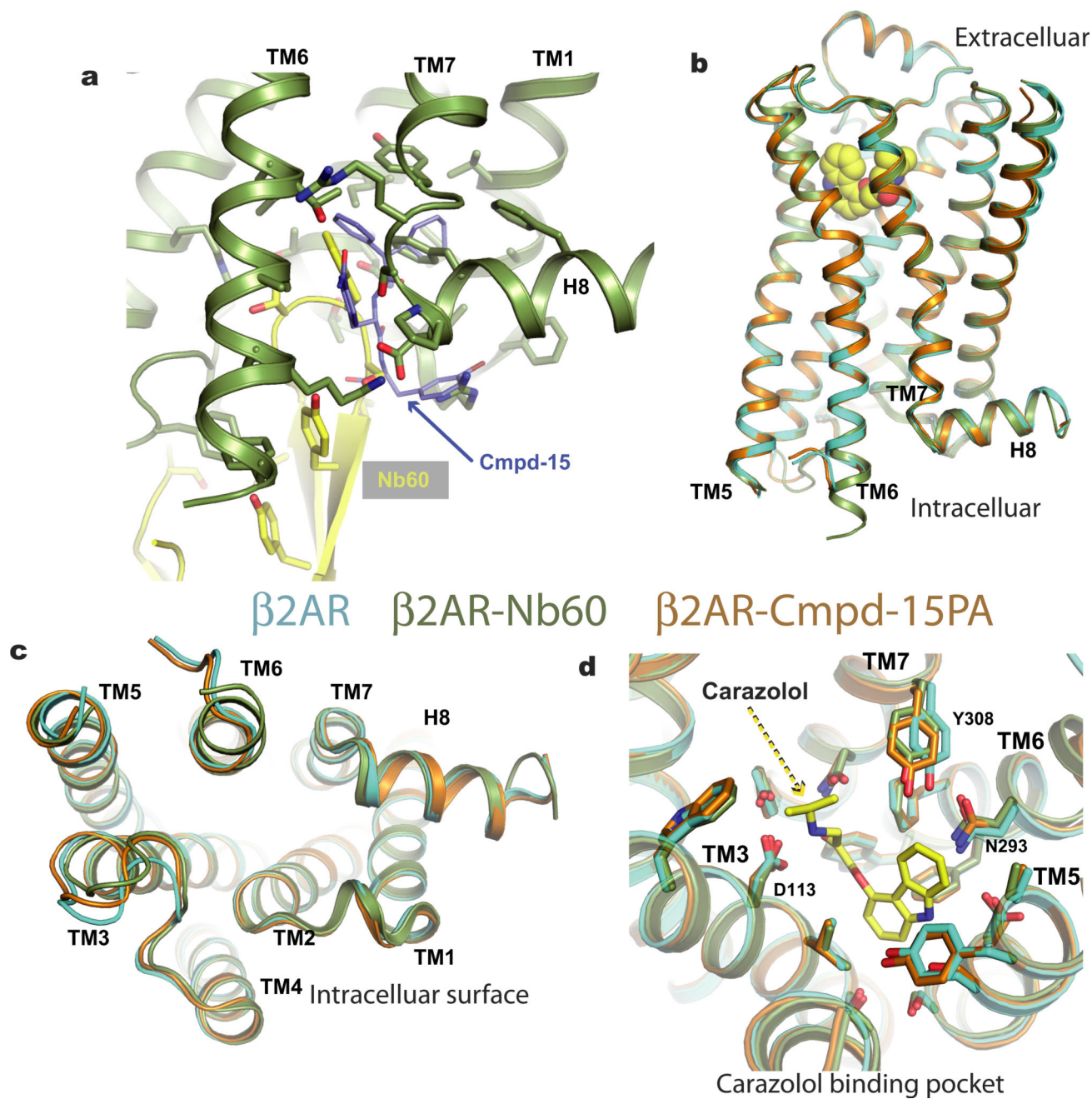
Extended Data Figure 6. Comparison of the structures of the \beta_2 AR (cyan, PDB, 2RH1), \beta_2 AR-Nb60 (green, PDB, 5JQH) and \beta_2 AR-Cmpd-15PA (orange) a , Cmpd-15PA binding pocket overlaps with Nb60 binding pocket. b-d , Different views of superimposed structures of the \beta_2 AR, the \beta_2 AR-Nb60 and the \beta_2 AR-Cmpd-15PA revealing very little structural difference associated with binding of Nb60 or Cmpd-15PA.
