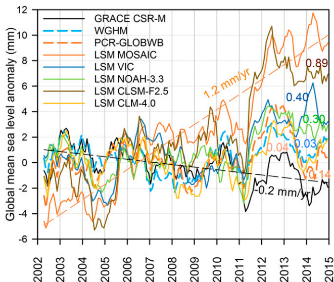
Fig. 7. GMSL change derived from TWSA trends for GRACE CSR-M, GHWRMs (PCR-GLOBWB and WGHM; dashed lines), and LSMs (MOSAIC, VIC, NOAH-3.3, CLSM-F2.5, and CLM-4.0). The black dashed line represents the downward contribution of GRACE CSR-M trends to GMSL, and the orange dashed line represents the upward contribution from LSM-MOSAIC. GRACE-positive TWSA trends ( 71 \text{ km}^3/\text{y} ) contribute negatively ( -0.2 \text{ mm}/\text{y} ) to GMSL, slowing the rate of rise of GMSL, whereas models contribute positively to GMSL, increasing the rate of rise of GMSL (Table 3).
