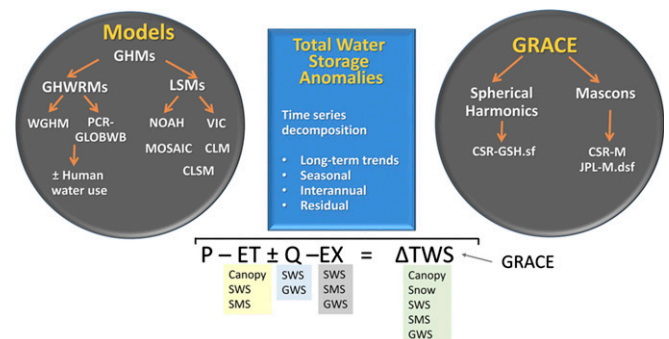
Fig. 2. Schematic depicting the data sources and analyses conducted in this study. See SI Appendix for acronyms. The water budget equation includes input from precipitation (P, snow and rain) and simulated output fluxes, including ET, runoff (Q), and extraction (EX). The storage compartments from which the fluxes derive include CWS, SWS, and SMS; Q from SWS; human EX from SWS and GWS; and residual total water storage (TWS), including all storages. Change in TWS ( \Delta\text{TWS} ) is calculated as a residual, accumulating errors from all of the fluxes. GRACE estimates change in TWS more directly.
