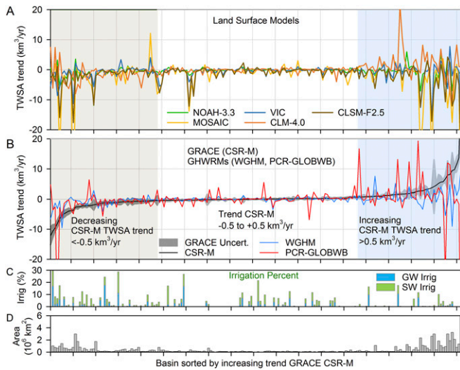
Fig. 4. (A–D) TWSA trends ranked according to trends from GRACE CSR-M from decreasing trends (buff background, \leq -0.5 km 3 /y) and increasing trends (blue, \geq 0.5 km 3 /y). The black line in B represents GRACE CSR-M TWSA trends, and the gray-shaded area represents uncertainty (Uncert.) in TWSA trends (SI Appendix, section 4.2). Irrig, irrigation.
