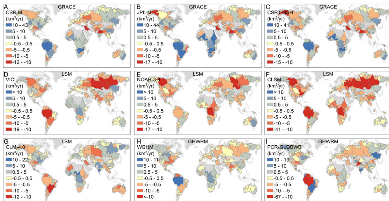
Fig. 3. TWSA trends expressed in volume (cubic kilometers per year) from three GRACE solutions: CSR-M (A), JPL-M.dsf (B), and CSR-Tellus-gridded spherical harmonic with scaling factor (CSRT-GSH.sf) (C); four LSMs: VIC (D), NOAH-3.3 (E), CLSM-F2.5 (F), and CLM-4.0 (G); and two GHWRMs: WGHM (H) and PCR-GLOBWB (I). Output from MOSAIC is not shown because of space restrictions.
