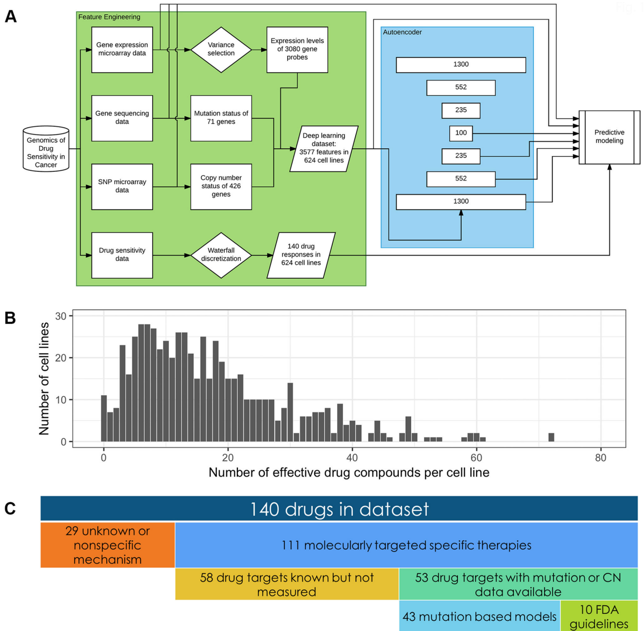
Figure 1. Drug sensitivity prediction workflow utilizing GDSC data
