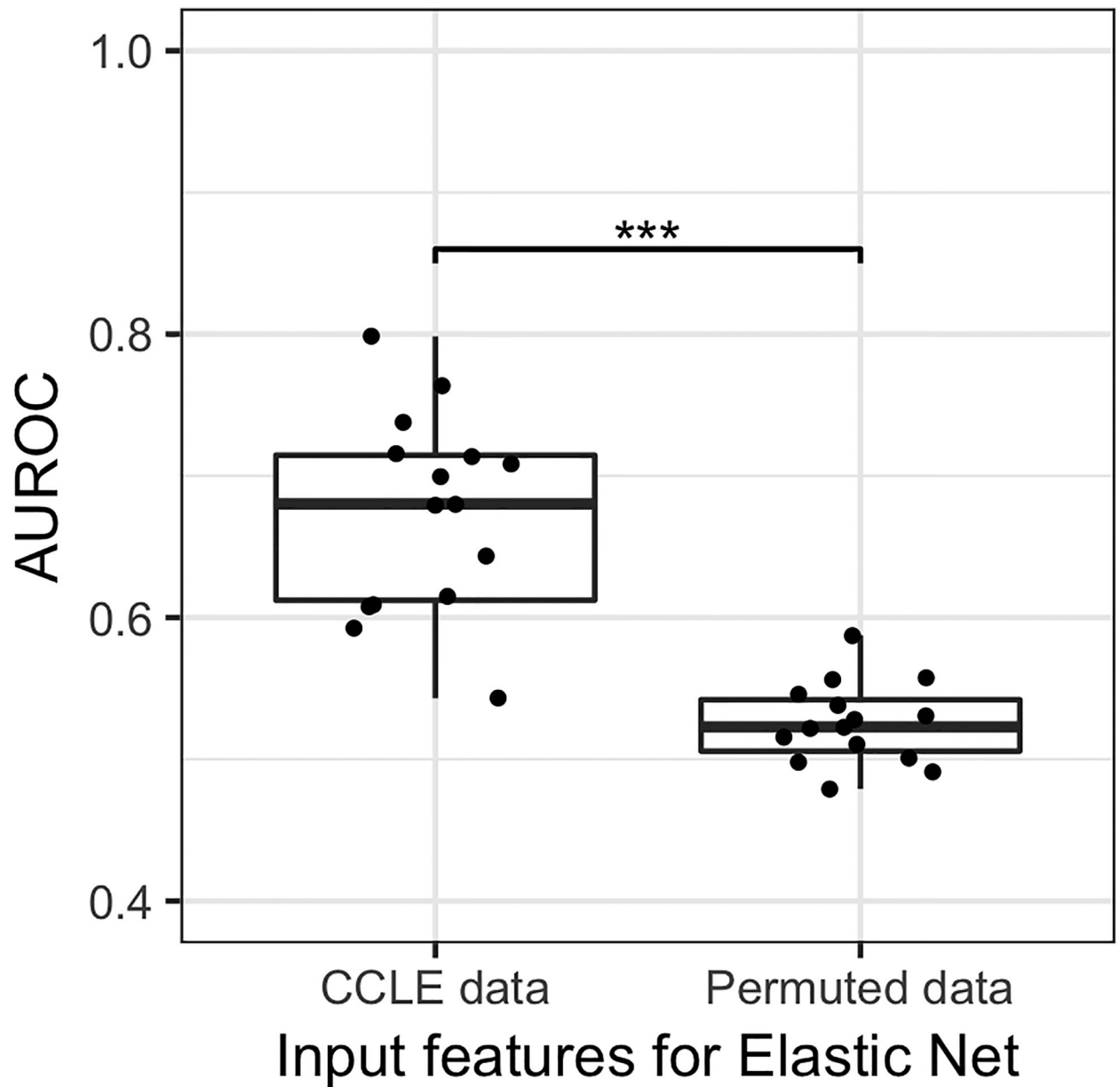
Figure 6. External validity of predictive models
