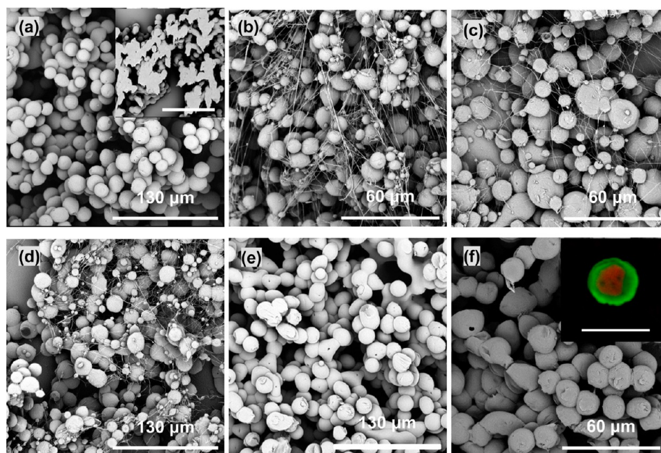
Figure 1. Products of the co-electrospraying of immiscible and miscible core/shell solution combinations: (a) PCL/chloroform (9 wt %) only, (b) PCL/chloroform (9 wt %) + water as core, (c) PCL/chloroform (9 wt %) + PEO/water (1 wt %), (d) PCL/chloroform (9 wt %) + PEG/water (15 wt %), (e) PCL/chloroform (9 wt %) + cyclohexane, and (f) PCL/chloroform (5 wt %) + PEG/chloroform (15 wt %). Co-electrospraying settings: applied voltage, 9 kV; working distance, 20 cm; core/shell flow rate, 0.5/2 mL/h (except in part f, where the core/shell flow rate was 1.0/3.0 mL/h). Insets in parts a and f: cross-section of electrospayed solid PCL microspheres (scale bar: 130 \mu\text{m} ) and a confocal laser scanning microscope image showing the core-shell structure (scale bar: 10 \mu\text{m} ), respectively. Spheres in these SEM images were collected on a static wire electrode placed above the aluminum foil substrate.
