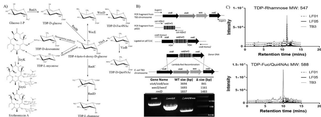
Figure 2. Metabolic pathway engineering to improve erythromycin formation. A) Competing pathways to desosamine and mycarose that were deleted in strains LF01 and LF05. B) Chromosomal gene deletion schematic ( vioA/vioB/wzx deletion example) and verification by PCR. PCR bands represent the expected deletion fragments of indicated knockouts. C) Deoxysugar assessment by LC-MS supporting metabolic engineering design.
