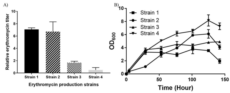
Figure 3. Erythromycin production across different strains. Relative erythromycin titer (A; measure at final time point) and optical density at 600 nm (OD 600 ; B) comparison. Strain 1: TB3 (pBPJW130/pBPJW144/pJM03/pJM02/pGro7); Strain 2: LF01(pDEBS/pTailoring); Strain 3: TB3(pDEBS/pTailoring); Strain 4: LF05(pDEBS/pTailoring). Error bars represent standard deviation values from three independent experiments.
