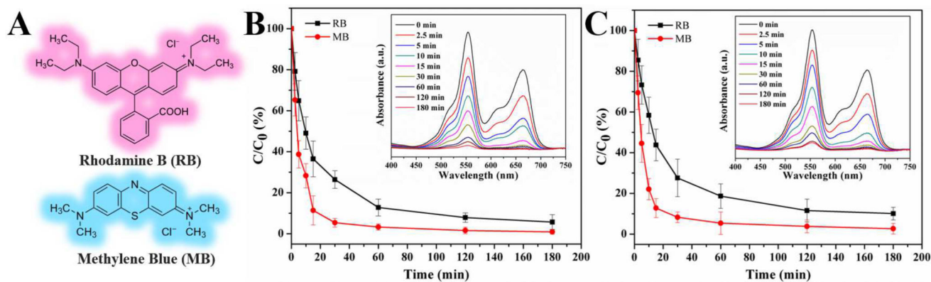
Figure 4. Adsorption of Rhodamine B (RB) and Methylene Blue (MB). (A) Chemical structures of RB and MB. (B–C) Adsorption rates of the mixture of RB and MB by WMSN (B) and EMSN (C). C_0 is the initial concentration of the RB and MB solution (Both at 10^{-5} M), and C is the concentration of that at different time intervals during the adsorption. Error bars show the standard deviations from three independent tests. The insets in (B) and (C) are a group of UV–vis spectra for time-dependent adsorption of RB and MB in the presence of WMSN and EMSN, respectively.
