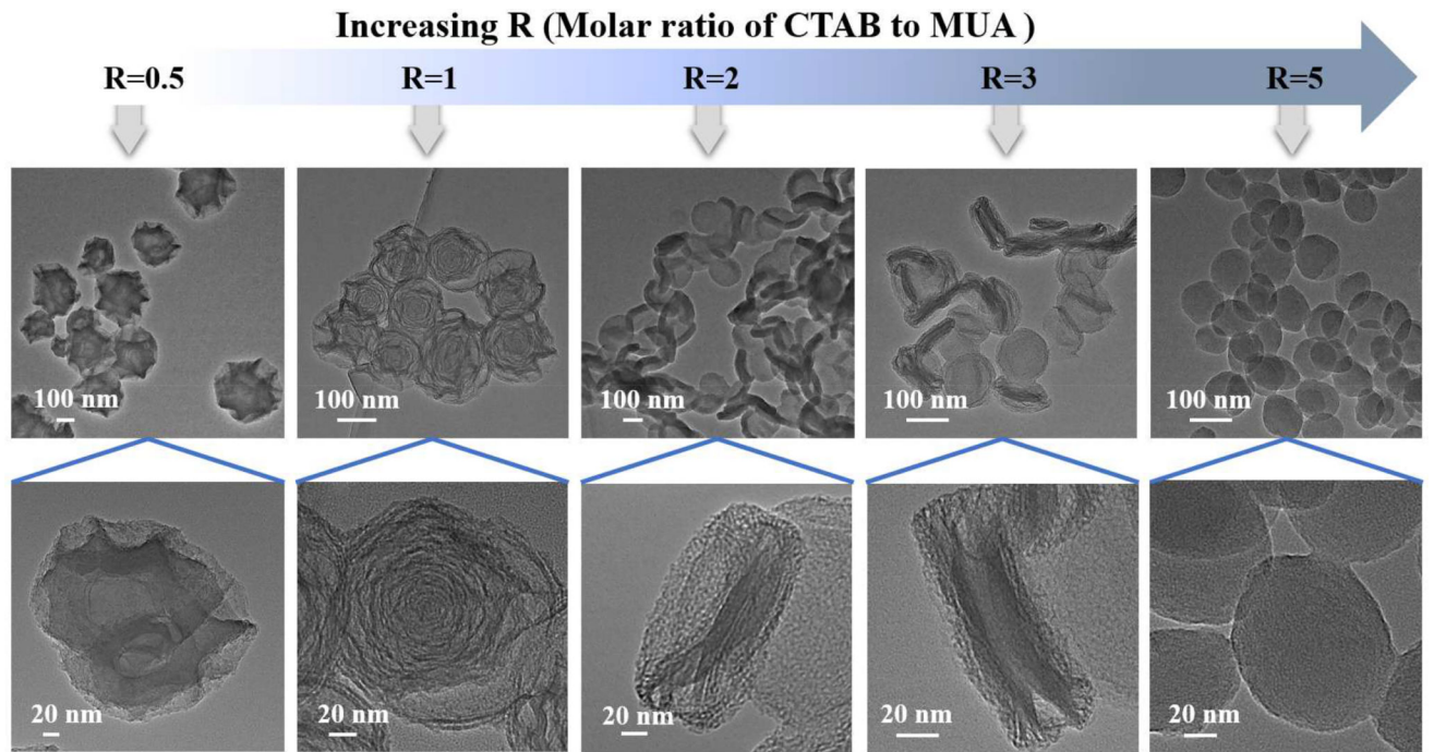
Figure 2. The effect of the molar ratio of CTAB to MUA on the morphology change of MSN.
