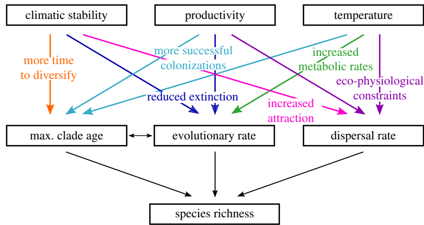
Figure 1. Theoretical framework depicting the relationships, and the underlying hypotheses, between evolutionary, ecological, climatic stability and richness variables. max., maximum.
