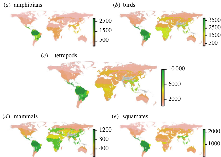
Figure 2. Global species richness maps. Species richness was computed by bioregion for (a) amphibians, (b) birds, (c) tetrapods, (d) mammals and (e) squamate reptiles.
