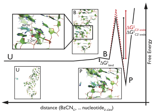
Figure 3. Hypothetical mechanism of RNA modification by SHAPE reagent. Schematic profile, where the free energy depends on the distance between reactive carbon ( C^* ) of BzCN reagent and O_{2'} oxygen from particular nucleotide. Insets represent snapshots of SRP–RNA motif with BzCN in unbound state (U), bound state in close proximity from 2' -OH group (B, highlighted in double-inset), and anticipated reaction adduct after the acylation reaction (P). Bound states are here defined as structures for which the distance between C^* and O_{2'} is <4.0 Å. Water molecules and counterions are not shown for clarity. We find that the barrier for binding ( \Delta G_{\text{bind}}^{\ddagger} ) and unbinding is marginal ( \sim 1 kcal/mol, Figure S11) in comparison with the activation barrier of the acylation reaction (estimated \sim 20 kcal/mol; see the SI part 4 for details). The activation free energy could be affected by some structural factors, for example, by the sugar pucker of the particular nucleotide in a reaction complex with reagent (in the range of a few kcal/mol favoring C2' -endo sugar pucker in a free energy; Table S2 in the SI).
