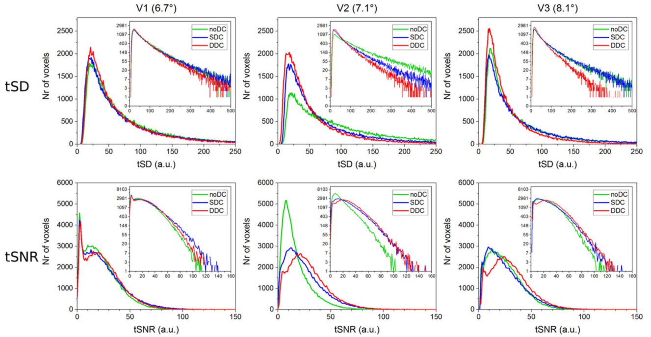
Fig. 5. Histograms comparing tSD (top row) and tSNR (bottom row) in a whole brain volume between EPI with noDC, SDC and DDC, where there was intentional motion (rotations up to 6.7°, 7.1° and 8.1° for V1, V2 and V3 respectively). Insets in the upper right corner of each graph show the same results on a logarithmic scale.
