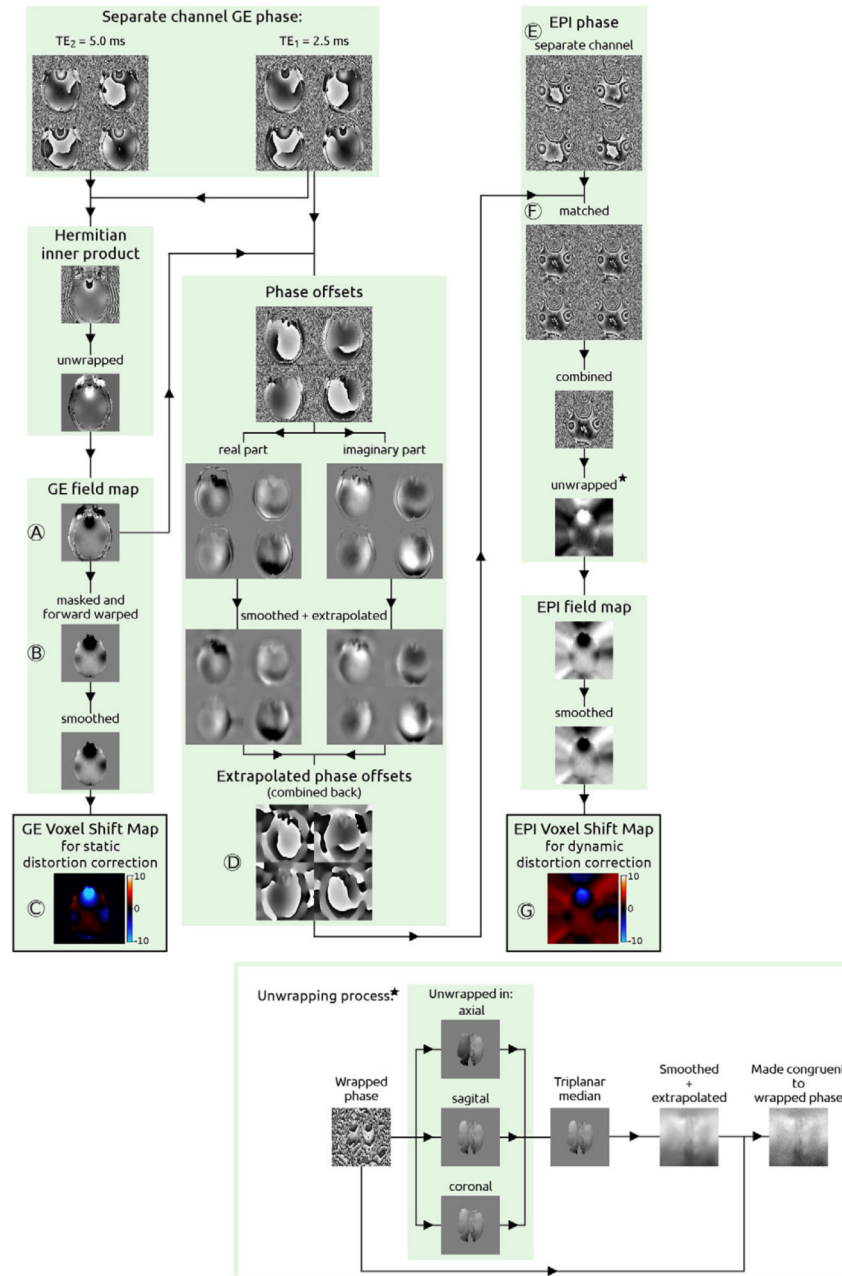
Fig. 1. Processing steps used in Exp. 3 to obtain voxel shift maps used for the SDC and DDC of EPI proposed here. For simplification, 4 out of 32 channels are shown. At the bottom right of the image unwrapping steps applied to the EPI phase (but not to GE phase) are presented. Capital letters (A–G) mark the steps described in the text.
