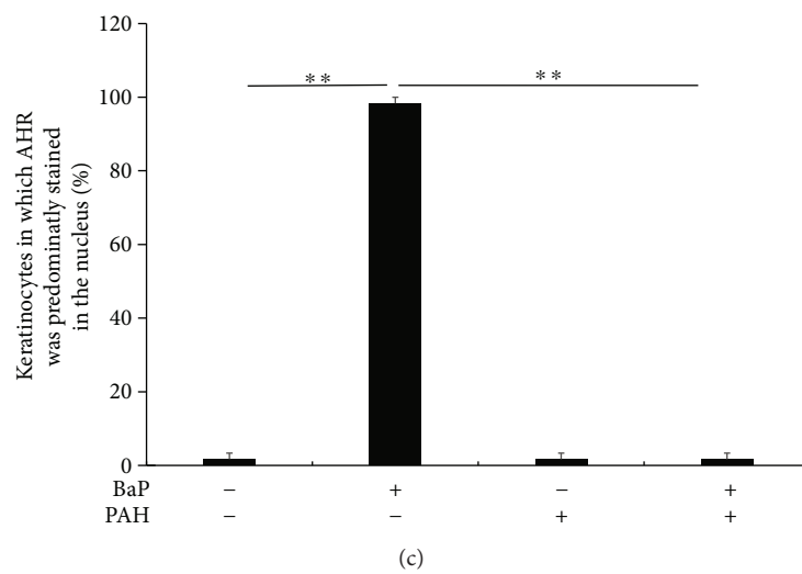
FIGURE 1: (a) HaCaT keratinocytes were treated with BaP in the presence or absence of PAH (1, 10, 100, or 1000 μM), and CYP1A1 expression was measured by quantitative RT-PCR. * p < 0.05 . ** p < 0.01 . (b) Subcellular localization of AHR was visualized by immunofluorescence. Cells were stained with anti-AHR antibody (green) and 4',6-diamidino-2-phenylindole (blue). BaP induced cytoplasmic to nuclear translocation of AHR, which was blocked by PAH. (c) The proportion of keratinocytes in which AHR was predominantly stained in the nucleus was calculated. ** p < 0.01 .
