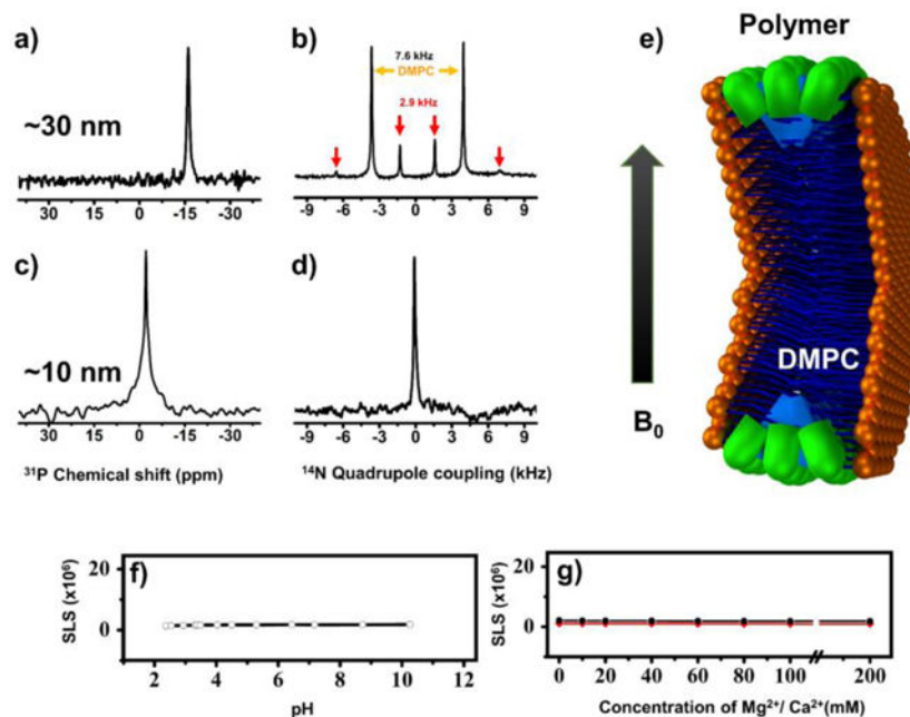
Figure 4. SMA-QA nanodiscs exhibit magnetic-alignment and remarkable tolerance to pH and divalent metal ions
