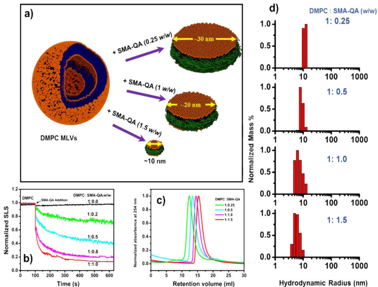
Figure 2. Formation and size tunability of SMA-QA lipid nanodiscs
