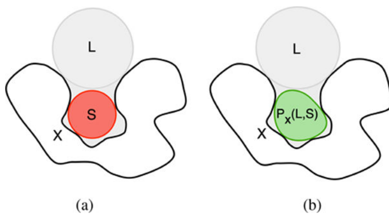
Figure 11. Detecting cavities using GHECOM [Kaw10]: (a) representation of the molecular surface (X), a small probe (S) in a cavity, and a large probe (L) on the protein surface; (b) cavity as given by P_X(L,S) .
