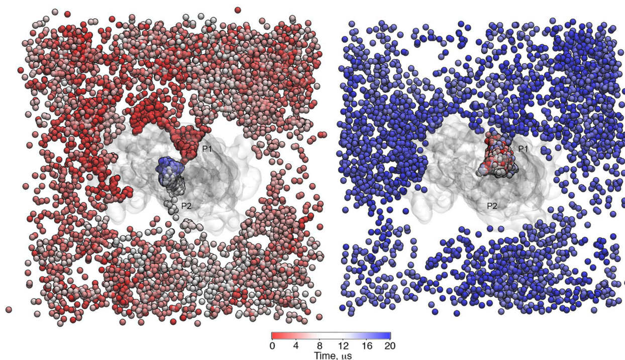
Figure 1. Two examples of \text{PO}_4 bead trajectories found in the pure POPS bilayer. (Left) At 0 \mu\text{s} , the lipid molecule resides outside of the cavity. It accesses the cavity twice during the simulation time, first during the first microsecond of the simulation through P1 and then after \sim 9 \mu\text{s} through P2. (Right) The selected lipid molecule remains inside the cavity for \sim 16 \mu\text{s} before exiting through P1. P-gp is shown as a transparent surface, and the \text{PO}_4 bead of the selected lipids is shown as a sphere, colored as a function of time.
