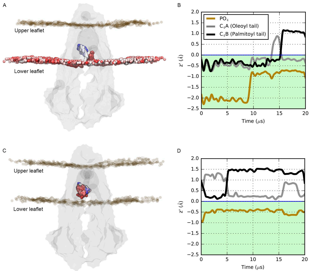
Figure 5. Dynamics of headgroups and tails inside the cavity of P-gp. (A–D) The mean z coordinate profile for the headgroup beads ( \text{PO}_4 ) and tail beads ( \text{C}_{4A} and \text{C}_{4B} ) plotted over 20 \mu\text{s} of simulation for a lipid that accesses the cavity two times (A and B) and a lipid that remains in the cavity (C and D). In A and C, P-gp is shown in the gray surface, and the position of the selected \text{PO}_4 bead is shown as a colored sphere, from red to white to blue, as a function of time following the color map in Fig. 1. The z profiles of the \text{PO}_4 bead (brown line) and the \text{C}_{4A} and \text{C}_{4B} beads (gray and black lines) were calculated over windows of 1 \mu\text{s} .
