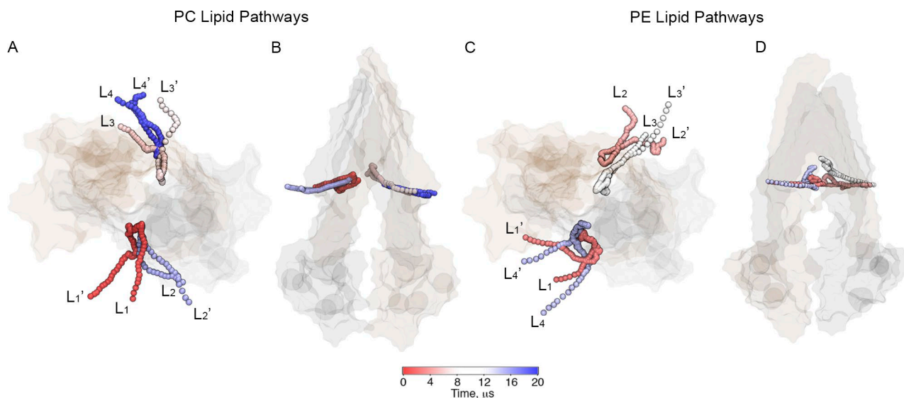
Figure 7. Lipid pathways found for PC and PE lipid types in plasma membrane ratio PC/PE. Different lipid headgroups (PO 4 beads) access the cavity of P-gp through both portals as a function of time during the 20- \mu s simulation. (A and B) Two different views of PC lipid pathways. (C and D) Two different views of PE lipid pathways. P-gp is shown in a transparent surface representation. Each lipid shown is labeled in the order in which it accesses the cavity along the simulation by subindex i = [1, \dots, 4] . Before accessing the cavity, the lipids are labeled as L i ; after leaving the cavity, the lipids are labeled as L i '.
