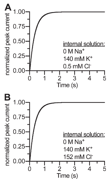
Figure A4. Turnover rates are independent of internal \text{Cl}^- concentration. (A) Simulated peak current recovery experiment using 140 mM internal K^+ and 0.5 mM internal \text{Cl}^- . (B) Same protocol as in A, but using 152 mM internal \text{Cl}^- . The simulations reproduce data described in Hasenhuetl et al. (2016).
