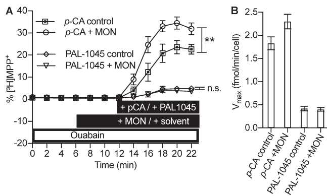
Figure 7. Substrate release by p -chloroamphetamine and PAL-1045. (A) Release of [ 3 H]MPP + from preloaded HEK293 cells expressing SERT. [ 3 H]MPP + release is plotted as percent [ 3 H]MPP + over time. The experimental conditions are indicated in the black bars: 3 μM p -chloroamphetamine (open squares), 3 μM p -chloroamphetamine + 10 μM monensin (open circles), 3 μM PAL-1045 (open diamonds), and 3 μM PAL-1045 + 10 μM monensin (open triangles). 100 μM ouabain (open bar) was present starting at t = -40 min and throughout the experiment. For statistical analysis, the total area under the curve after basal release (i.e., fractions t = 0 to t = 4 min) was calculated for each individual trace. **, P < 0.01; n.s., not significant. One-way ANOVA followed by Bonferroni's multiple comparison test. (B) Calculated [ 3 H]MPP + release rate for one cell in femtomole/minute (= V max ). (A and B) Data are means ± SD, n = 8–9 independent observations per condition.
