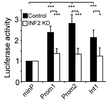
Figure 8. The \alpha -TAT1 gene contains functional CARG boxes. (A) Schematic representation of the \alpha -TAT1 gene with an indication of the putative CARG boxes (CARG elements 1–4) present in the region examined and the fragments (Prom1, Prom2, and Int1) used in our analysis. (B) The indicated constructs were transfected in control and INF2 KD RPE-1 cells. The luciferase activity was measured and was expressed relative to that of cells transfected with minP. (C) The four CARG boxes present in the constructs Prom1, Prom2, and Int1 were placed in tandem upstream from a minimal promoter ( \alpha -TAT1 CARGs1–4). A similar construct was made in which the four central nucleotides of each box were mutated in such a way that all of them were C or G ( \alpha -TAT1 CARGs1–4m). Control cells were transfected with the indicated constructs in the presence or absence of the MRTF-A \Delta N100 construct, and the luciferase activity of the cells was assayed. The histogram represents the luciferase activity obtained in each case relative to that of cells transfected with minP. Data in B and C represent the mean and SEM of seven and four independent experiments, respectively; ns, not significant; *, P < 0.05 ; **, P < 0.01 ; ***, P < 0.001 .
