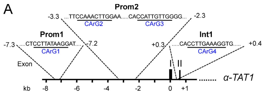
Figure 8. The \alpha -TAT1 gene contains functional CARG boxes. (A) Schematic representation of the \alpha -TAT1 gene with an indication of the putative CARG boxes (CARG elements 1–4) present in the region examined and the fragments (Prom1, Prom2, and Int1) used in our analysis. (B) The indicated constructs were transfected in control and INF2 KD RPE-1 cells. The luciferase activity was measured and was expressed relative to that of cells transfected with minP. (C) The four CARG boxes present in the constructs Prom1, Prom2, and Int1 were placed in tandem upstream from a minimal promoter ( \alpha -TAT1 CARGs1–4). A similar construct was made in which the four central nucleotides of each box were mutated in such a way that all of them were C or G ( \alpha -TAT1 CARGs1–4m). Control cells were transfected with the indicated constructs in the presence or absence of the MRTF-A \Delta N100 construct, and the luciferase activity of the cells was assayed. The histogram represents the luciferase activity obtained in each case relative to that of cells transfected with minP. Data in B and C represent the mean and SEM of seven and four independent experiments, respectively; ns, not significant; *, P < 0.05 ; **, P < 0.01 ; ***, P < 0.001 .
