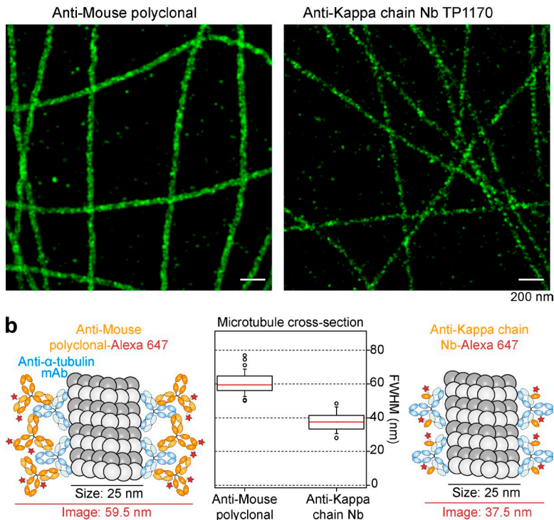
Figure 6. STORM imaging with anti- \kappa chain nanobody TP1170. (a) BS-C-1 cells were stained with an anti- \alpha tubulin monoclonal antibody (IgG1 \kappa ) and detected with Alexa Fluor 647-labeled goat anti-mouse polyclonal antibody or Alexa Fluor 647-labeled anti-mouse \kappa chain nanobody TP1170. STORM images of the two samples show subdiffraction limit organization of the tubulin filaments. (b) To quantify the effect of the label size on the apparent width of the filaments in the STORM images, averaged cross-sectional profiles of straight segments of filaments from the two samples were measured. First, the two labeling approaches are illustrated on the left and right of the figure, showing the expected smaller width for the nanobody labeling case. In the middle, box plots illustrate the results of the width analysis (boxes indicate first and third quartiles of data values, whereas the red line indicates the median value; error bars indicate the 10th and 90th percentiles). In these measurements, the median width of the tubulin filaments decreased by a significant amount (from 59.5 to 37.5 nm) when stained with the anti-mouse \kappa chain nanobody TP1170.
