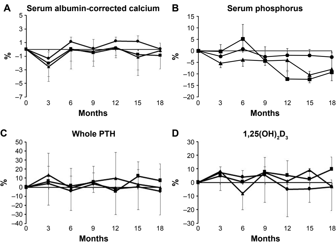
Figure 1 Percent changes of calcium metabolism for 18 months after denosumab therapy. Notes: Percent changes in serum albumin-corrected calcium (A), serum phosphorus (B), serum whole PTH (C), and serum 1,25(OH) 2 D 3 (D) for the 18-month study period. Circles show the TNF group, triangles show the TCZ group, and rectangles show the ABT group. Abbreviations: ABT, abatacept; PTH, parathyroid hormone; TCZ, tocilizumab; TNF, tumor necrosis factor inhibitors.
