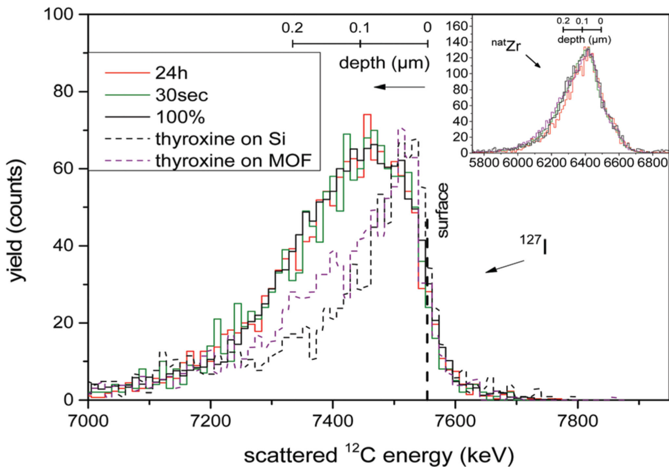
Fig. 2. Normalized RBS signal of the iodine content and normalized RBS zirconium signal (inset). The vertical dashed line marks the surface of the sample, while the lower energies correspond to the depth of the sample with the corresponding depth scales depicted. The solid lines correspond to UiO-66@Si samples that have been exposed to PSE for times as indicated, 100% is the (UiO-66-(I-bdc)@Si) sample, and the dotted lines correspond to reference samples with thyroxine.
