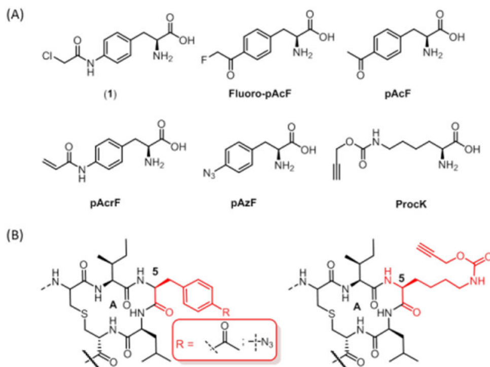
Figure 3. (A) ncAAs used in this study (B) Biorthogonal chemical handles incorporated into Ser5TAG NisA.
