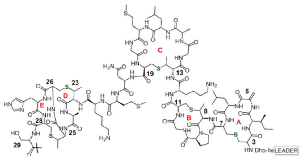
Figure 1. Wild type mNisA. Highlighted thioether rings and key residues for this study (residues 30-34 omitted for simplicity).
