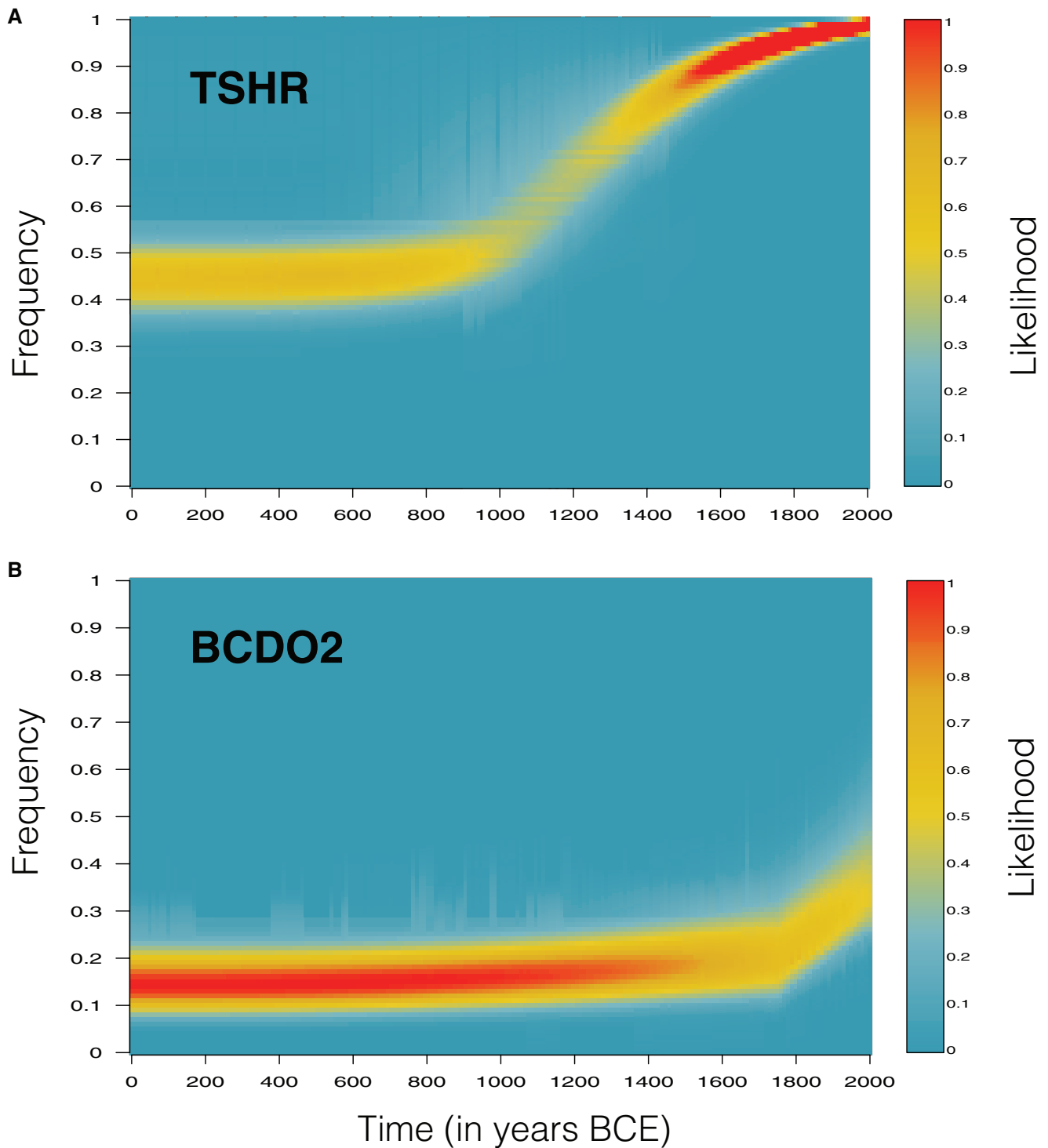
Fig. 2. Posterior distribution of the derived allele frequency as a function of time for the TSHR locus (a) and the BCDO2 locus (b). The likelihoods are color coded (see color bar) and are shown relative to the maximum likelihood in the plot.
