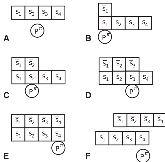
Fig. 4. First phase of Mechanism (C): Polymerization of the complementary polynucleotide chain R_L^{\bar{S}} catalyzed by a primordial polymerase P^\pi .
