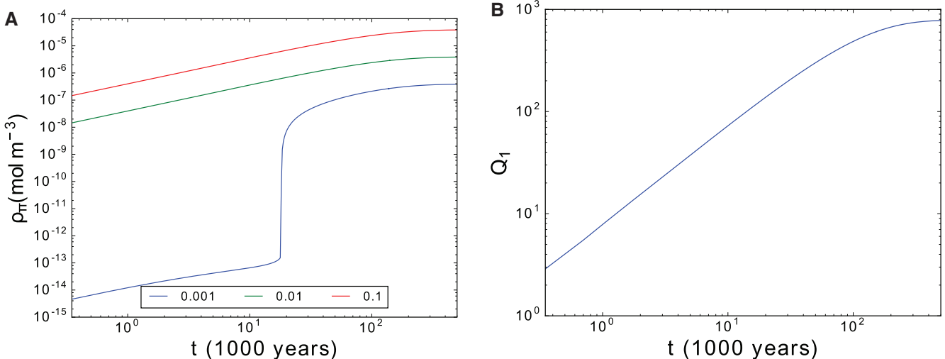
Fig. 5. (a) Time evolution of the polymerase for initial concentration \rho_r = \rho_p = 0.001, 0.01 , and 0.1 \text{ mol m}^{-3} . (b) Q_1 for initial concentration \rho_r = \rho_p = 0.01 \text{ mol m}^{-3} . Parameter values: K_p^- = 4 \times 10^{-11} \text{ s}^{-1} , Z = 10^6 \text{ mol}^{-1} \text{ m}^3 \text{ s}^{-1} , \lambda = 0.15 .
