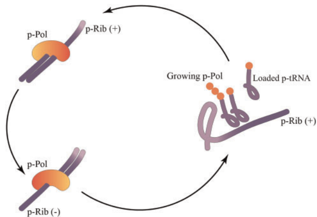
FIG. 6. The nucleopeptide Initial Darwinian Ancestor. In this cartoon model, a short strand of XNA has the functionality of both a primordial p-mRNA and a p-Rib. Primitive XNA molecules loaded with amino acids (p-tRNA) bind to the p-Rib via codon–anticodon pairing. This allows adjacent amino acids to undergo peptide bond formation and a short peptide chain is produced. A certain peptide sequence is able to act as a primordial XNA-dependent XNA polymerase (p-Pol) able to copy both + and – p-Rib strands to eventually produce a copy of the p-Rib(+) strand.
