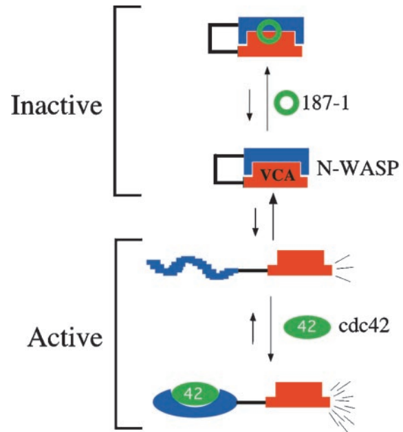
Fig. 4. A model for the inhibition of N-WASP by 187-1. Native N-WASP exists predominantly in a “closed” inactive conformation. Whereas binding to cdc42 stabilizes the “open” active conformation, 187-1 stabilizes the autoinhibited state. Competitive binding of 187-1 and cdc42 to N-WASP, therefore, drives the equilibrium between autoinhibited and activated states, respectively.
