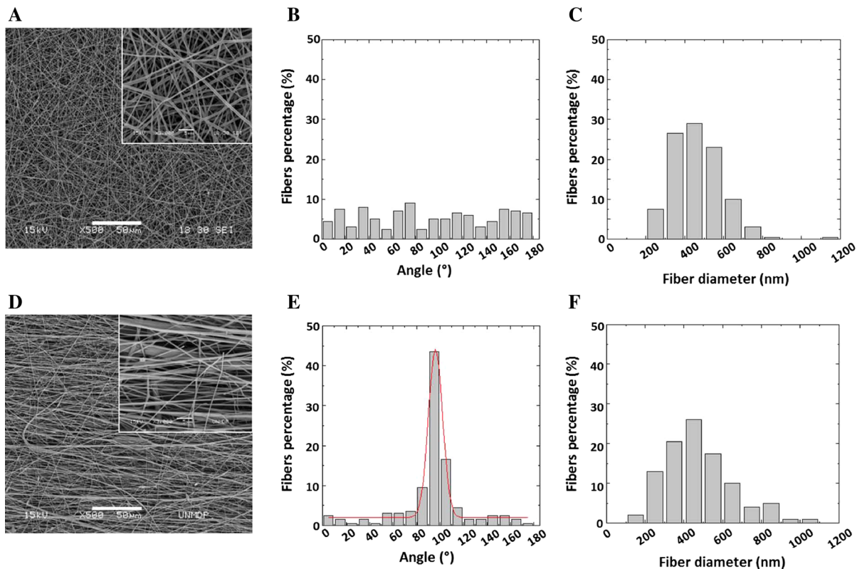
Fig. 4 Nanofiber topography analysis. a–c Scanning electron microscopy ( a ), fiber alignment ( b ) and fiber diameter ( c ) in random poly (L-lactic acid) scaffolds. d–f Scanning electron microscopy ( d ), fiber alignment ( e ) and fiber diameter ( f ) in aligned poly (L-lactic acid) scaffolds at 1175 rpm. Please note that the difference in topography of scaffolds with aligned
