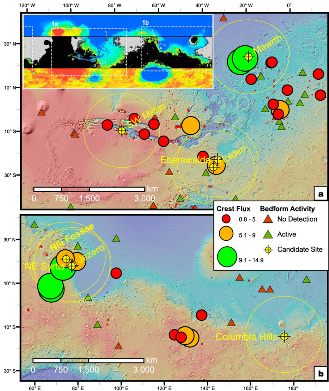
Figure 1. Subarea maps of candidate-landing sites with results from global bedform monitoring efforts and regional sand flux measurements for (a) western and (b) eastern hemispheres. Sand dune crest flux measurements (graduated circles grouped in three classes with units of \text{m}^3 \text{m}^{-1} \text{yr}^{-1} ; see Table S1). The 1,000 km radius ellipses centered on candidate sites provide scale. Base map is Mars Orbiter Laser Altimeter (MOLA) shaded relief with colored elevation from +4 to -5 km. The distribution of dune fields (red polygons) is provided as mapped by Hayward et al. (2014) and Chojnacki et al. (2014, 2017). Figure 1a inset provides a MOLA
