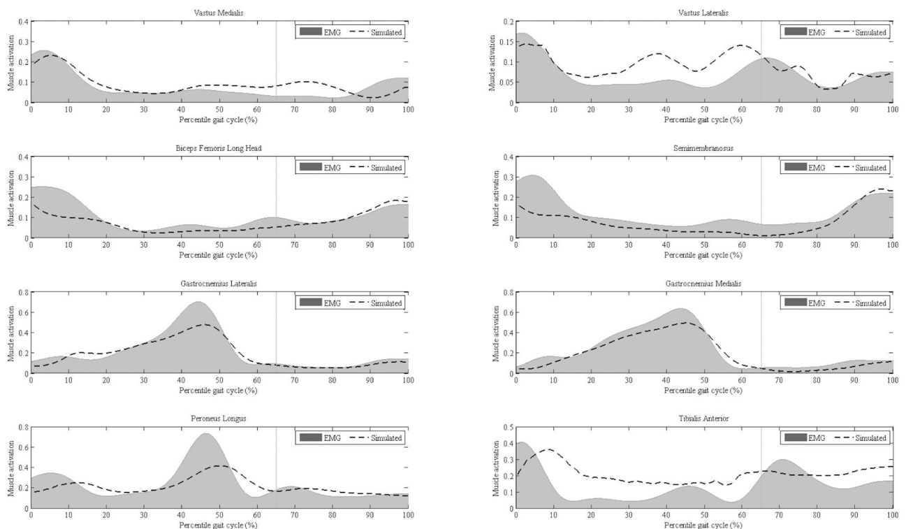
Fig 2. Simulated muscle activations compared to measured EMG for the lower limb muscles (starting from heel strike to the end of swing phase). The vertical solid line denotes the timing of toe-off.
