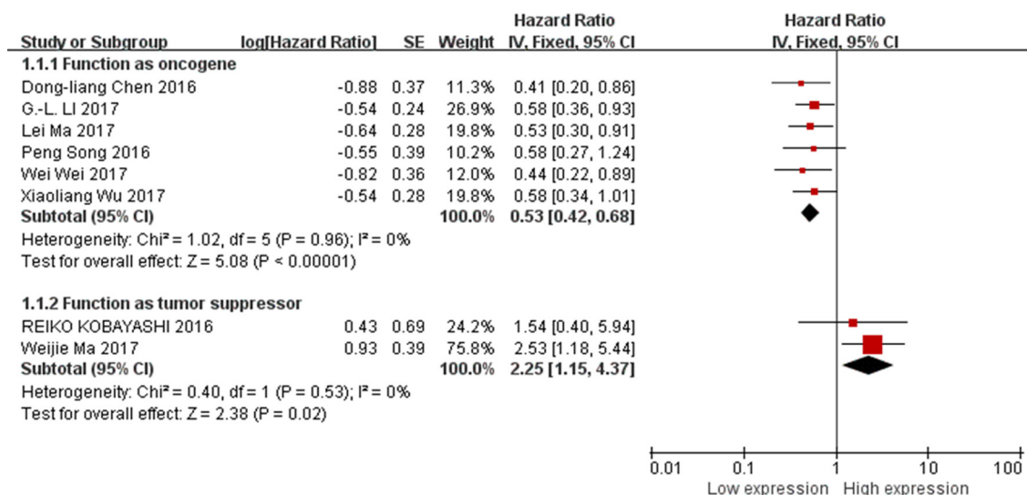
Figure 2: Forest plot for the association between XIST expression levels with OS.
