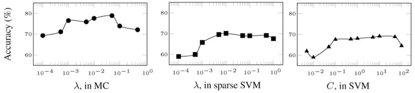
Fig. 8. Accuracy of the competing methods, as a function of their hyperparameter.
