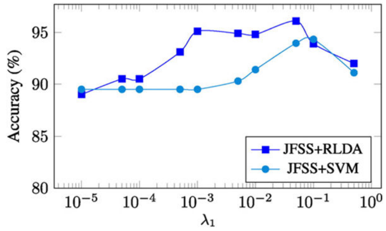
Fig. 5. Accuracy as a function of the JFSS hyperparameter ( \lambda_1 ), experimented on synthetic data, with \rho=100 .
