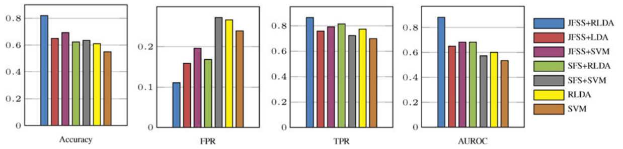
Fig. 6. Comparisons of results by the proposed (JFSS + RLDA) and the baseline methods.
