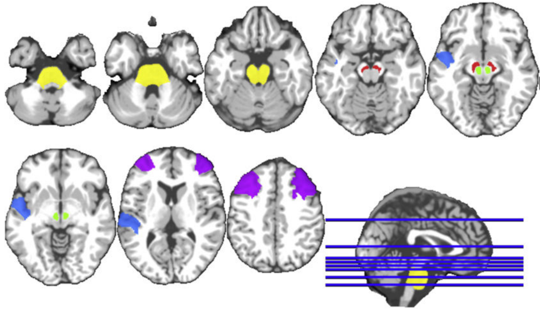
Fig. 9. Top and most frequent selected ROIs by our method.
