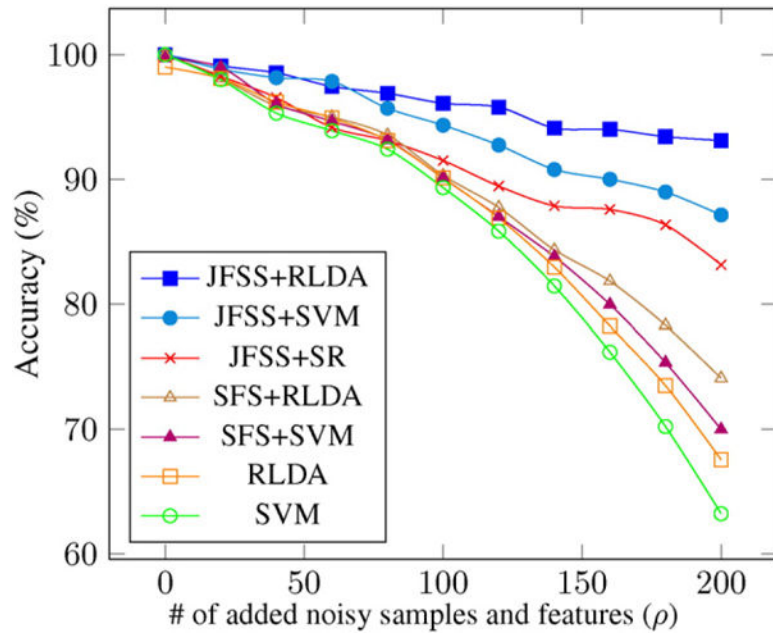
Fig. 4. Comparisons of results on synthetic data, for three different runs. The diagram shows the mean accuracy for different methods as a function of \rho .
