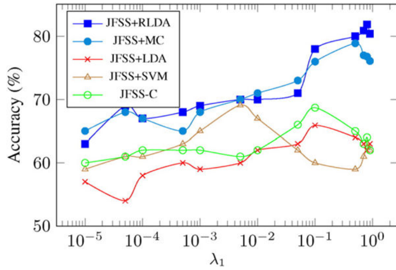
Fig. 7. Accuracy as a function of the JFSS hyperparameter ( \lambda_1 ), for the Parkinson's disease diagnosis experiment.
