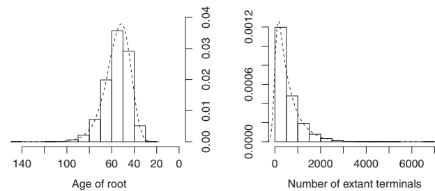
Fig. 1. Parametric bootstrapping of a diversification process. The primate phylogeny of Springer et al. (2012) was fit to a birth-death model (pxbdfit). To explore the breadth of plausible diversification outcomes the maximum likelihood parameters (b: 0.339487, d: 0.268944) were used to simulate (pxbdsim) 25 000 phylogenies conditioned on either the extant diversity (367, left) or root age (66.7066 Ma, right) of the empirical tree
