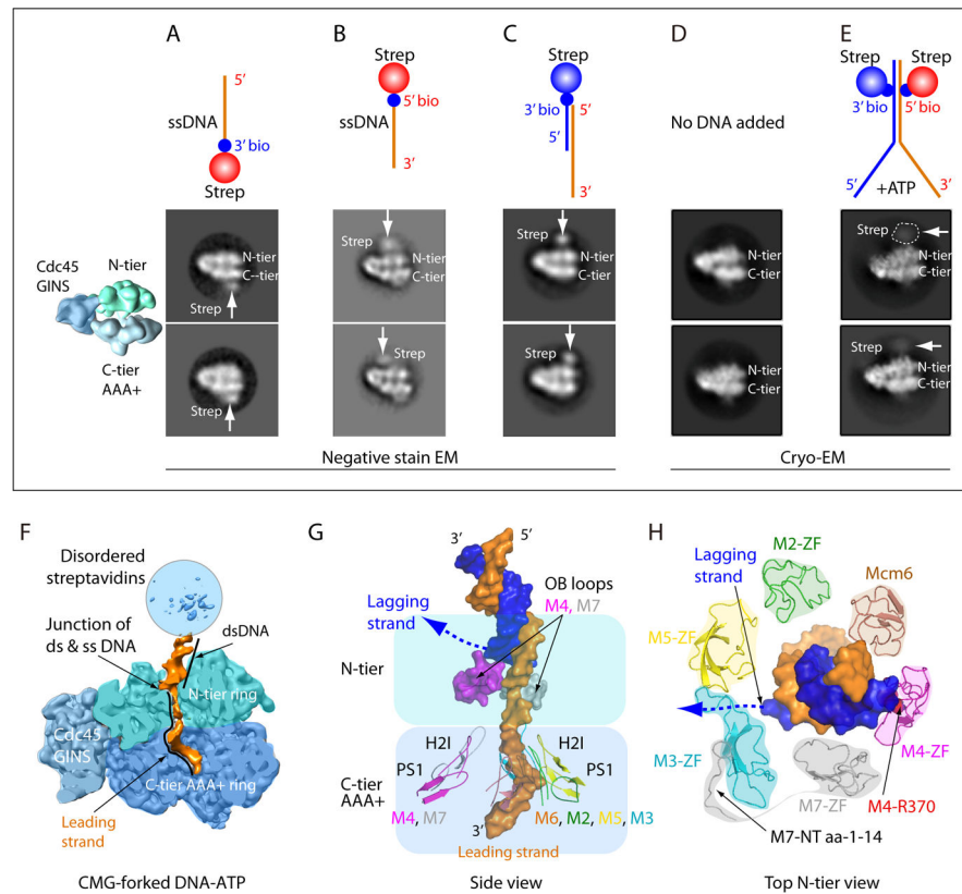
Figure 4. CMG-forked DNA structure with N-tier leading the C-tier during translocation A–C) Negative stain EM side views of CMG with streptavidin tipped oligos; colored diagram at left illustrates the tiers of Mcm2-7 and Cdc45/GINS. A) 20mer ssDNA 3' streptavidin. B) 20mer ssDNA 5' streptavidin. C) fork lacking a lagging strand and tipped with streptavidin on the ds end. D) CryoEM of CMG without DNA. Note the density of Mcm6 WHD protruding from the C-tier. E) CryoEM of CMG-forked DNA and ATP; CMG is stopped at the streptavidin blocks which are visible as a fuzzy (mobile) region. F) Cut away view through CMG-forked DNA illustrating dsDNA enters the top of the N-tier (light green) and leading ssDNA proceeds into the motor C-tier (blue). G) The DNA-interacting loops of Mcm2-7. Note that the upper OB loops of Mcm4 and Mcm7 block the lagging strand DNA. Inside the C-tier motor ring, the PS1 and H2I loops of Mcm 2, 3, 5, 6 spiral around and interact with the right-handed leading strand DNA coil; the corresponding loops in Mcm 4, 7 do not interact with DNA. Lagging ssDNA is not visible but a possible path is suggested by the dotted line. H) Top view of N-terminal ZF domains of Mcm2-7 binding the dsDNA. Note dsDNA tilts toward and interacts with ZFs of Mcm 7, 4, 6. The Mcm3 ZF has an unusually long loop that forms the base between ZFs of Mcm 3, 5. The ordered N-terminal peptide of Mcm7 warps around and pulls Mcm3 ZF from Mcm5 ZF, creating a gap through which the lagging strand may escape (dotted line). The EM images and illustrations in panels A–E are adapted with permission from Figs 5 and 6 of 23 .
