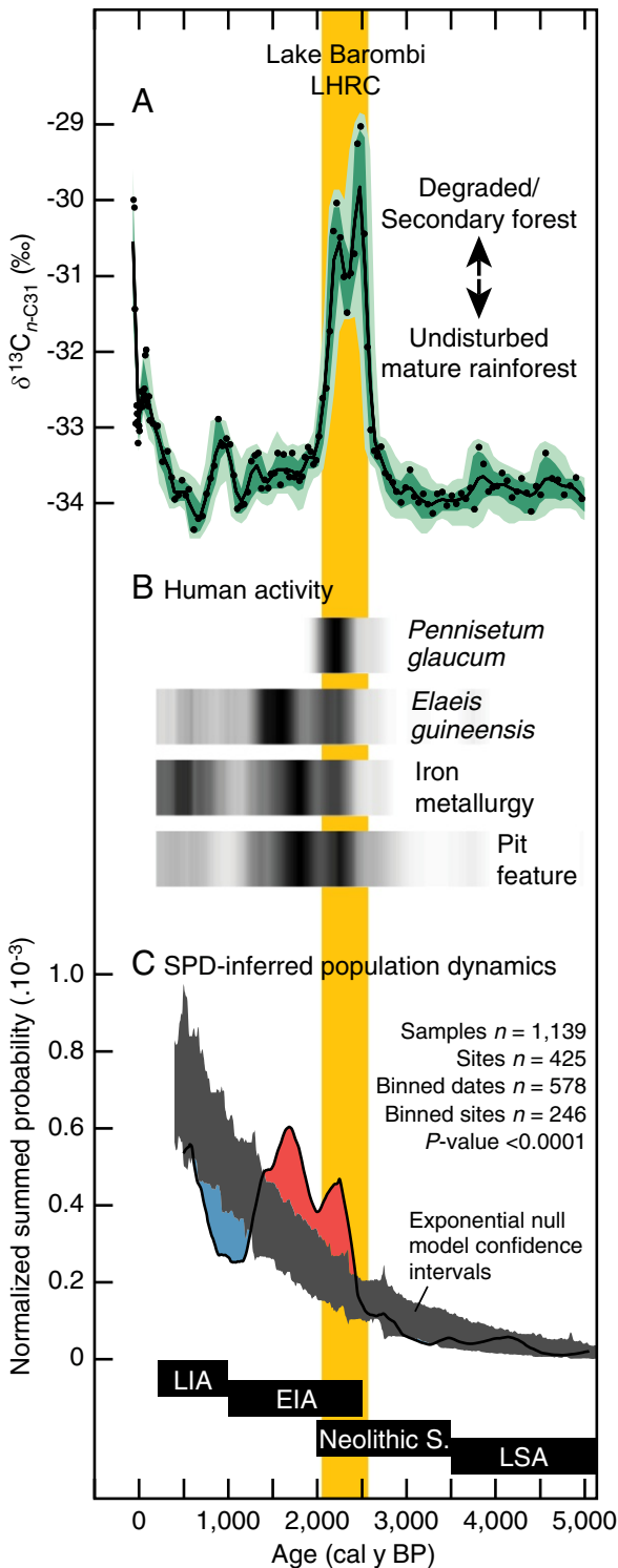
Fig. 4. Detailed comparison of the Lake Barombi vegetation changes and the archaeological record of WCA during the past 5,000 y. ( A ) Lake Barombi \delta^{13}\text{C}_{n-C31} indicating vegetation changes. \delta^{13}\text{C}_{n-C31} values have been corrected for the Suess effect for the last 160 y ( SI Appendix ). Dots are the raw measured data; line indicates median probability; envelopes reflect 68% (dark) and 95% (light) confidence intervals in the reconstruction, based on analytical and age model errors. ( B and C ) Archaeological synthesis of WCA. All presented archaeological data rely on the SPD of calibrated ^{14}\text{C} dates that were binned in space using 10-km radii and time using 200-y intervals ( SI Appendix ). SPDs were plotted with a 200-y moving average to prevent overinterpretation of smaller-scale variability (53–55) and are shown either as a gray scale [( B ) black represents maximum probability, white represents
